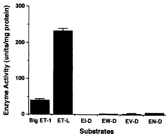
Fig. 3. Cleavage of Big ET-1 analogs by Immobilized Ovoidin column purified ECE. Peptide substrate concentration: 1.0 \times 10^{-5} M. To determine the concentration of the hydrolyzed fragments, standard curves were used for each peptide: ET-1 for Big ET-1, [D-Ile 20 ]ET-1[16–21] for EI-D, [D-Trp 21 ]ET-1[16–21] for EW-D and ET-1[16–21] for EV-D, EN-D and ET-L. Vertical bars indicate means \pm S.D. ( n = 3 ).
