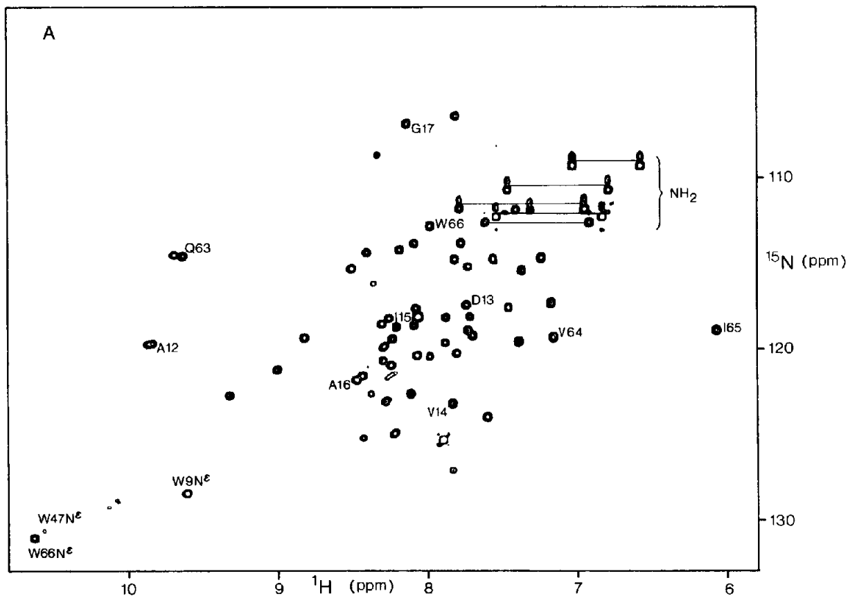
Fig.2. 600 MHz two-dimensional pure phase absorption ^{15}\text{N} - ^1\text{H} HMQC correlation (A) and relayed ^{15}\text{N} - ^1\text{H} HMQC-NOESY (B and C) spectra of Mu ner at 27°C. The ^{15}\text{N} (F1 axis)-NH(F2 axis) and ^{15}\text{N} (F1 axis)-aliphatic(F2 axis) regions of the relayed ^{15}\text{N} - ^1\text{H} HMQC-NOESY spectrum are shown in (B) and (C), respectively. Selected NH( i )-NH( i+1 ), \text{C}^\alpha\text{H}(i) -NH( i+1 ) and \text{C}^\beta\text{H}(i) -NH( i+1 ) NOE connectivities are shown in (B) and (C). The peaks in (A) and (B) are labelled at the position of ^{15}\text{N}(i) -NH( i ) connectivity; while those in (C) are labelled at the position of the ^{15}\text{N}(i) - \text{C}^\alpha\text{H}(i) or ^{15}\text{N}(i) - \text{C}^\beta\text{H}(i) connectivities, the latter being indicated by the letter \beta . The NOESY mixing time was 200 ms. Water suppression was achieved by pre-saturation during the relaxation delay and, in the case of the ^{15}\text{N} - ^1\text{H} HMQC-NOESY experiment, during the mixing time \tau_m as well. The sample contained 2.7 mM Mu ner in 90% \text{H}_2\text{O} /10% \text{D}_2\text{O} containing 150 mM sodium phosphate buffer, pH 7.0, with the protein ~93% ^{15}\text{N} labelled. 800 increments were recorded for each spectrum with 16 and 32 scans per t_1 value for the correlation and relayed-correlation experiments, respectively. The digital resolution is 9.8 Hz/pt in F2 and 4.1 Hz/pt in F1, the latter being obtained by appropriate zero filling. The spectra were recorded on a Bruker AM600 spectrometer. ^1\text{H} and ^{15}\text{N} chemical shifts are expressed relative to 4,4-dimethyl-4-silapentane-1-sulfonate and liquid \text{NH}_3 , respectively.
