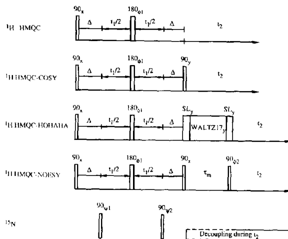
Fig.1. Pulse schemes for heteronuclear MQC correlation and relayed heteronuclear MQC-COSY, -HOHAHA and -NOESY experiments. Each of the four schemes utilizes the ^{15}\text{N} pulses shown at the bottom of the figure. The phases are cycled as follows: \phi_1 = 2(x), 2(-x) ; \phi_2 = 4(x), 4(y), 4(-x), 4(-y) ; \psi_1 = x, -x ; \psi_2 = x (and may be inverted together with the receiver phase after the basic phase cycle is complete); receiver (HMQC and relayed HMQC-COSY) = x, -x ; receiver (relayed HMQC-NOESY) = 2(x, -x), 2(y, -y), 2(-x, x), 2(-y, y) . The duration of \Delta was 4 ms, slightly shorter than 1/(2J_{\text{NH}}) . To obtain pure phase absorption spectra using the time proportional incrementation method [29] the phase of \psi_1 is incremented by 90^\circ for every successive t_1 value. ^{15}\text{N} decoupling during the acquisition time ( t_2 ) is achieved using the WALTZ-16 decoupling sequence [24]. In addition, to avoid effects of an incomplete steady state, the phase \psi_2 and the receiver phase may be inverted after completion of the above phase cycles [30].
