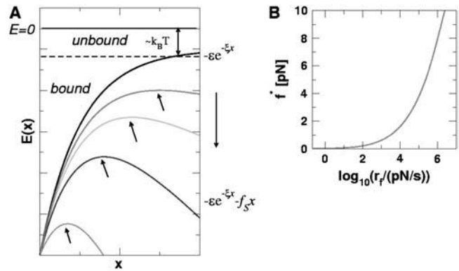
FIGURE 14 (A) Sketch of the one-dimensional potential E(x) as a function of x for several values of f_S . The transition-state location is obtained using E'(x_{\text{ts}}) = 0 . The boundary separating bound and unbound states is given by |E(x_{\text{ts}})/k_B T| = 1 . (B) Dependence of the most probable unbinding force f^* as a function of r_f . The ( f^* , \log r_f ) plot for the artificial potential is similar to that shown in Fig. 4 B.
