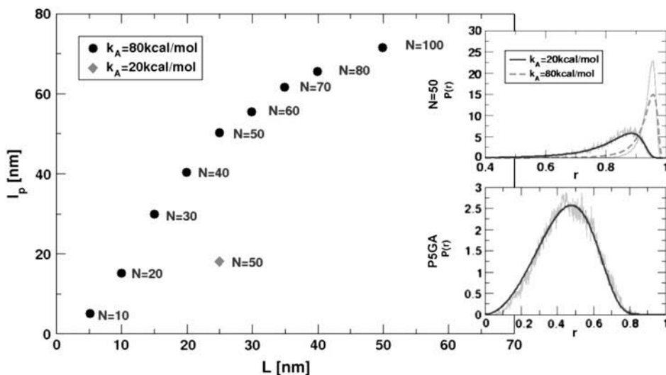
FIGURE 15 Persistence length l_p as a function of contour length L for linkers at 290 K. The number of monomers N (Eq. 9) is also shown. The values of l_p and L are obtained by fitting the end-to-end distance distribution function P(R) generated by simulations to the theoretical expression based on a mean field model (Eq. 23). An example of such a fit for a linker with N = 50 , using two different values of k_A (see Eq. 9), is shown in the top inset. For large N , l_p converges to a constant value. The fit of simulated P(R) for P5GA computed at T = 500 \text{ K} > T_m is shown in the bottom inset. From the WLC fit, we obtain l_p \approx 1.5 \text{ nm} and L = 12.5 \text{ nm} for P5GA.
