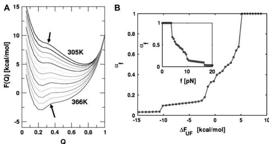
FIGURE 12 (A) Free energy profiles of Q at different temperatures. Note that the positions of the transition states over the temperature variation almost remain constant. (B) The movement of transition state measured in terms of the Leffler parameter (Eq. 17). The structural nature of a transition state is monitored by the free energy difference between NBA and UBA when f is an external variable. The inset shows the variation of \alpha with respect to force; value of T = 290 K.
