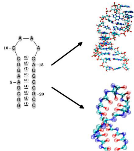
FIGURE 1 Coarse-grained representation of a molecule of RNA using three interaction sites per nucleotide—phosphate (P), sugar (S), and base (B). On the left we present the secondary structure of the 22-nt P5GA hairpin, in which the bonds formed between basepairs are labeled from 1 to 9. The PDB structure (17) and the lowest energy structure obtained with the coarse-grained model are shown on the right.
