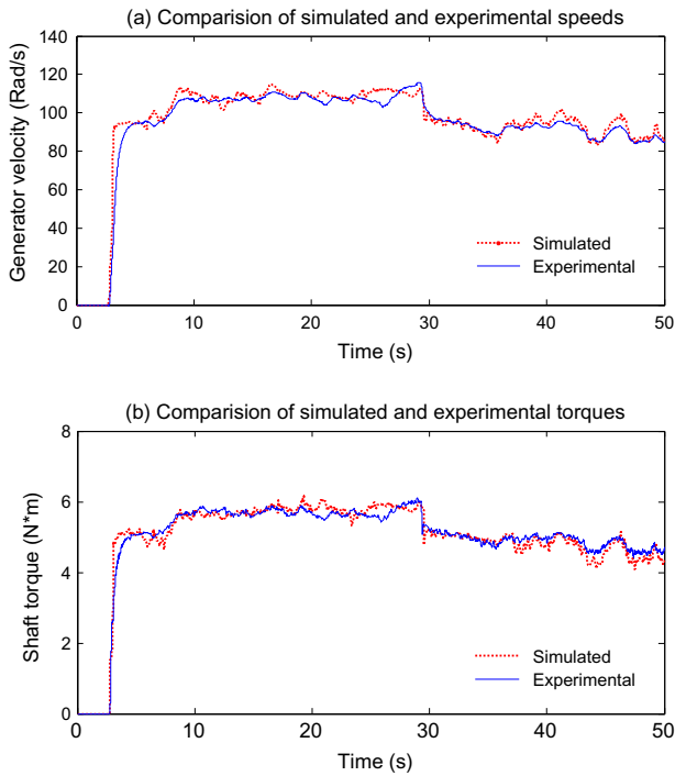
Fig. 16. Comparisons of the test results and the simulated data for the WTS.
