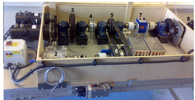
1 – DC motor (wind turbine simulator) 5 – Belt transmission system 2 – Scroll expander 6 – Clutch B 3 – Inertia plate 7 – Torque and speed meter 4 – Clutch A 8 – PMSG
