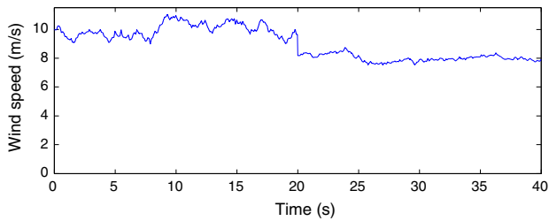
Fig. 10. Simulated wind speed profile.
