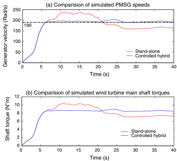
Fig. 11. Comparison of dynamic responses of the hybrid system with designed controllers connected and the stand-alone wind turbine without any control.
