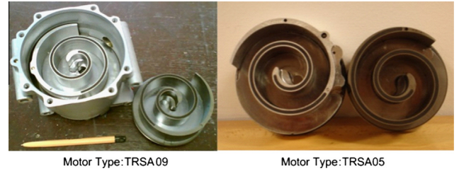
Fig. 3. Illustration of the scroll expander structure (manufactured by Sanden).
