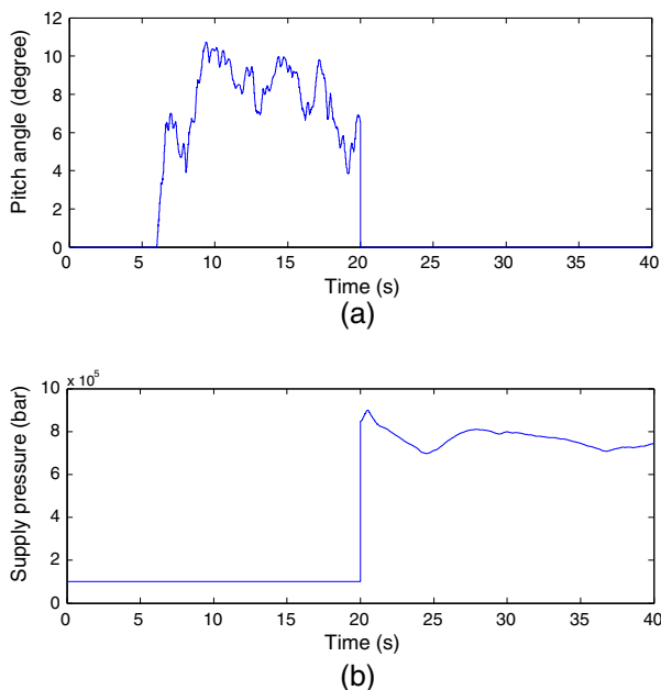
Fig. 12. Dynamic responses of the controlled variables in the hybrid system.
