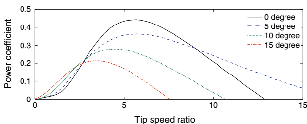
Fig. 2. Power coefficients as a function of tip speed ratio and pitch angle.
