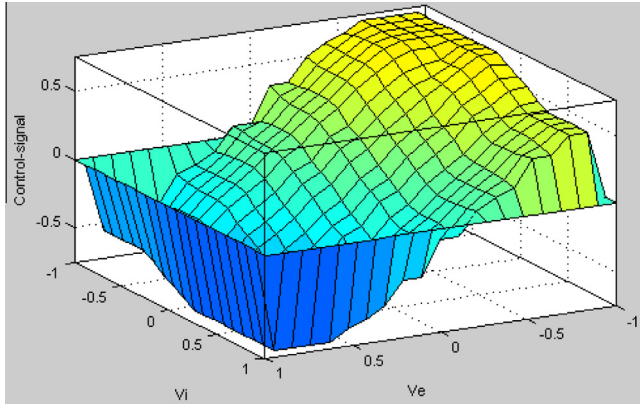
Fig. 8. Fuzzy logical controller nonlinear input & output map.
