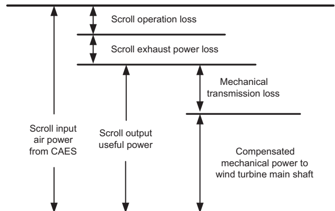
Fig. 18. Power transmission and conversion from the small-scale CAES to the wind turbine system.
