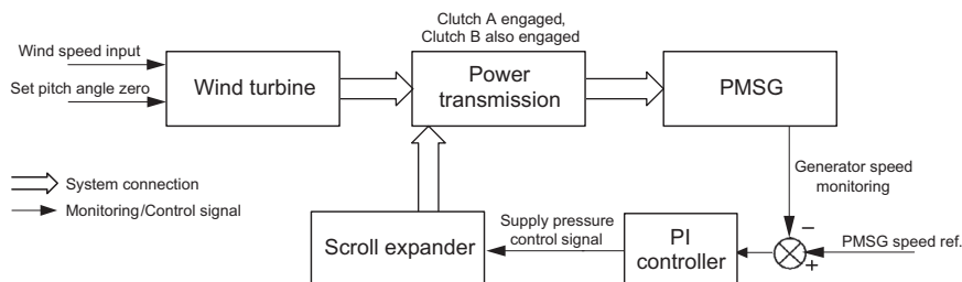
Fig. 9. Schematic of the scroll expander supply pressure PI control.
