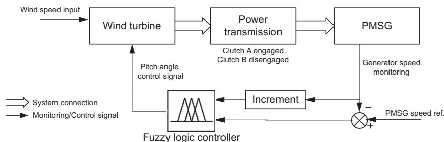
Fig. 7. Schematic of the pitch angle fuzzy logic control.
