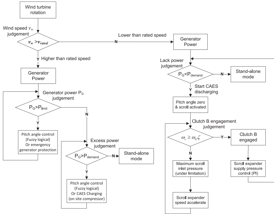
Fig. 6. Multi-mode control diagram for the proposed hybrid system.
