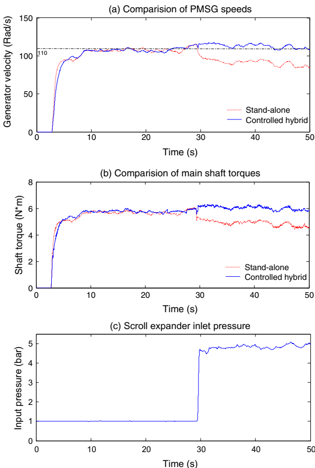
Fig. 17. Experimental test results of the stand-alone wind turbine and the controlled hybrid system.
