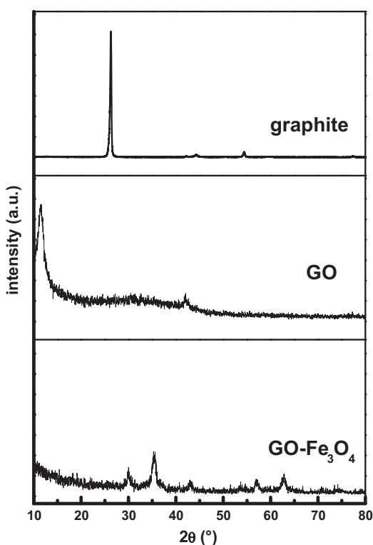
Figure 3 X-ray diffraction patterns of graphite powder (C), graphene oxide (GO) and magnetic graphene oxide nanocomposite (GO-Fe 3 O 4 ).
