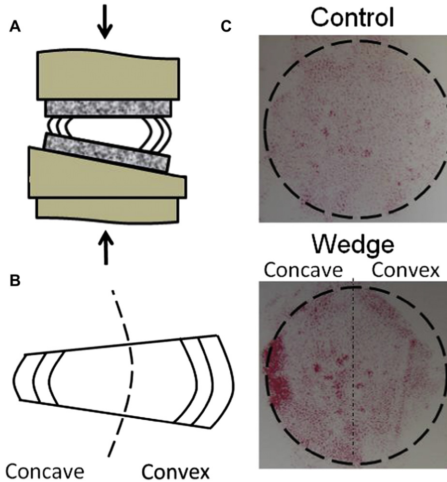
Fig. 1. (A) Loading schematic. (B) Concave/convex nomenclature. (C) Compressive stress distribution of both groups with a maximum compressive stress of \sim 0.45 MPa in the concave annulus.
