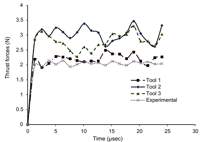
Fig. 14. Thrust forces during SPH simulation with new and worn tools.
