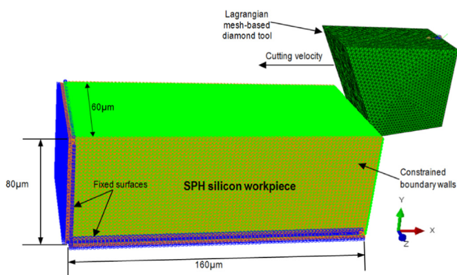
Fig. 13. SPH machining model of SPDT of silicon.
