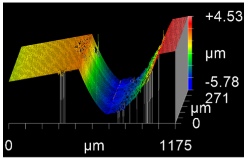
Fig. 8. Plunge cut surface with final brittle fracture.
