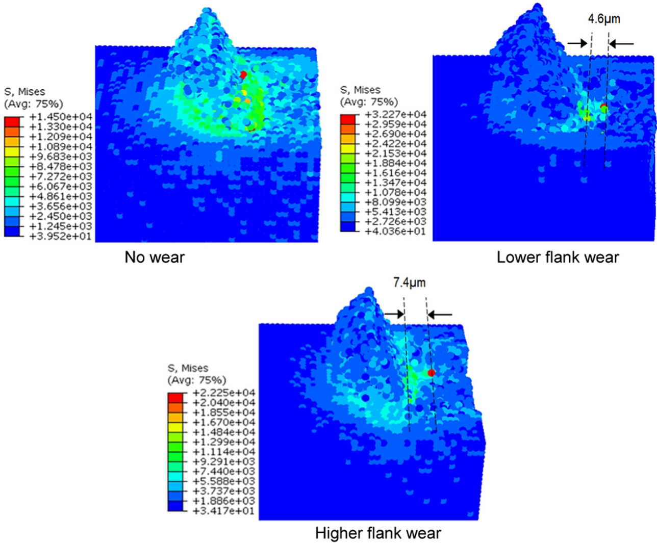
Fig. 15. Von Mises stress (MPa) distribution for different tool wear conditions.
