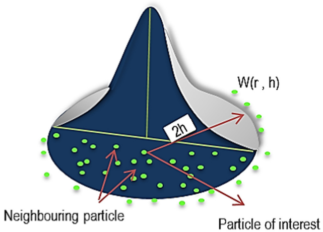
Fig. 11. SPH kernel approximation.
