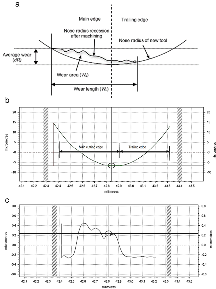
Fig. 3. Estimation of tool wear (a) schematic illustration of the tool edge recession (b) plunge profile of worn tool after 5 km (c) zoomed-in image showing worn area of the main cutting edge.
