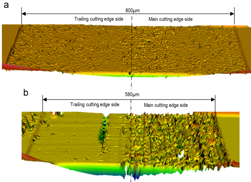
Fig. 10. Surface topography of (a) initial plunge cut and (b) final plunge cut.
