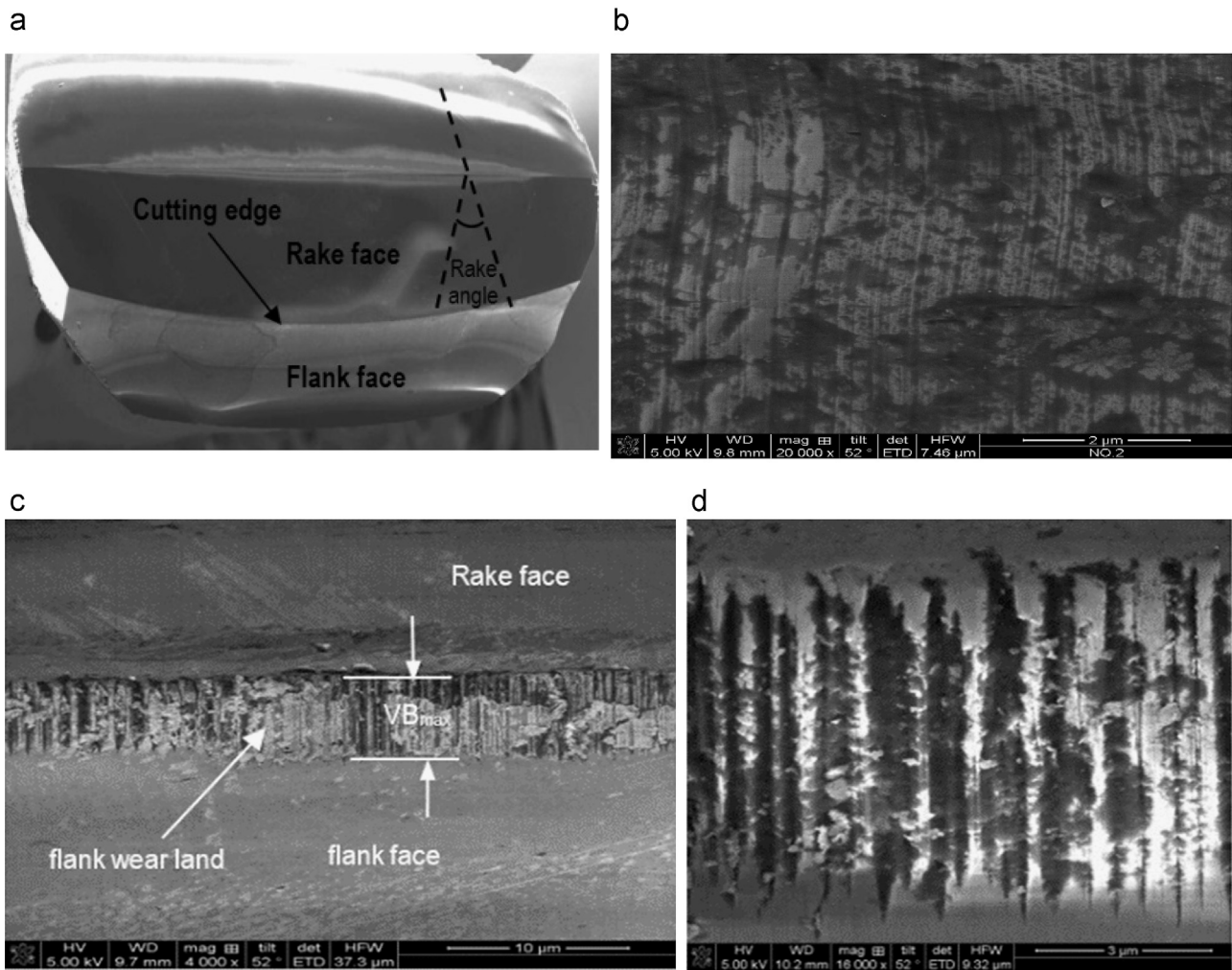
Fig. 2. SEM images of diamond tool (a) new tool (b) flank wear (after cutting distance of 5 km) (c) Final tool wear when brittle fracture appeared on silicon surface (d) zoomed image of (c) shows groove and abrasive wear mechanism.
