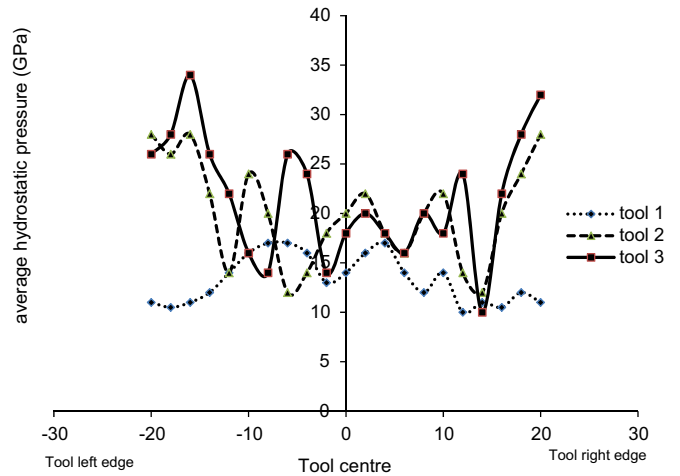
Fig. 17. Hydrostatic pressure distribution along the tool cutting edge.
