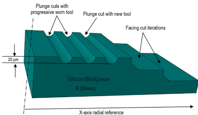
Fig. 1. Experimental SPDT plan details.
