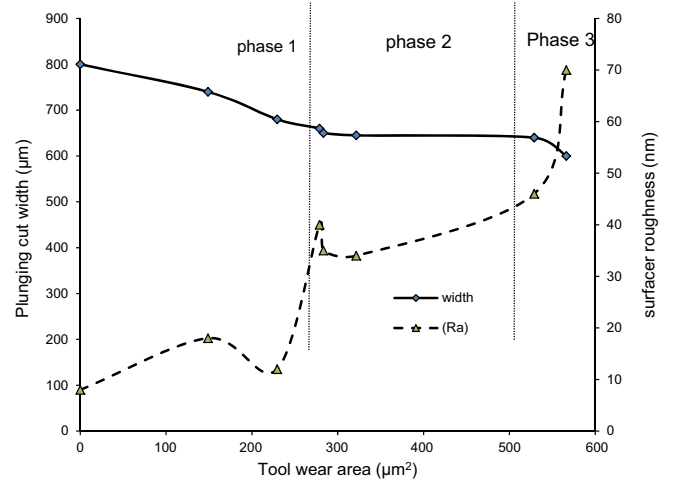
Fig. 9. Variation of plunging cut width and surface roughness with tool wear.
