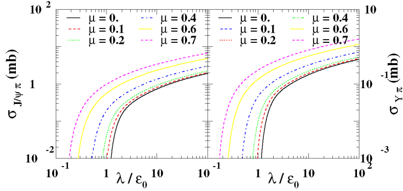
Fig. 3. J/\psi-\pi (left) and \Upsilon-\pi (right) total cross section as a function of the pion energy \lambda for various values of the screening parameter \mu .
