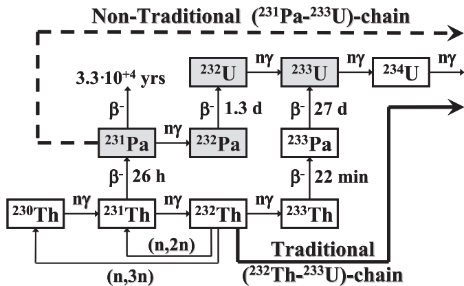
Fig. 1. Chains of nuclide transformations in the thorium–uranium fuel.
