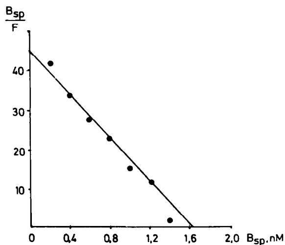
Fig. 3. Scatchard plot of binding of GMDP-Lys( ^{125}\text{I} Hp) to viable macrophages.
