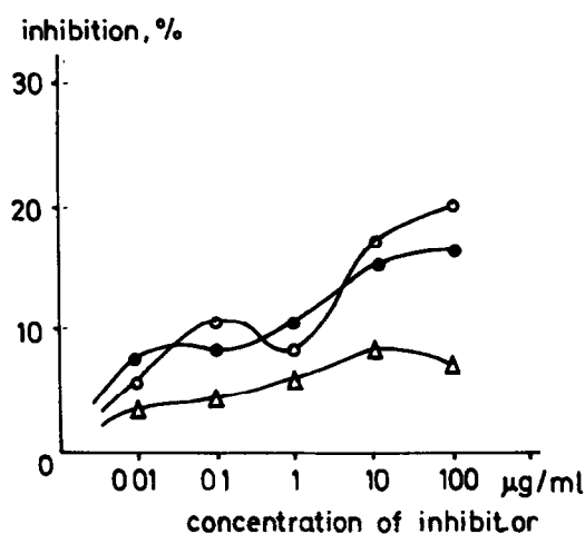
Fig. 2. Inhibition analysis of GMDP-Lys( ^{125}\text{I} Hp) binding to viable macrophages. Inhibition with GMDP (●), GMDP-Lys (○), L-GMDP (△).
