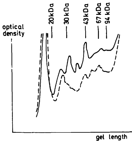
Fig. 5. Scan from the autoradiography film from SDS-PAGE of GMDP-Lys( ^{125}\text{I} AzS)-labeled permeabilized peritoneal macrophages.
