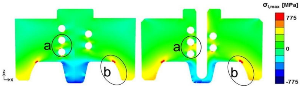
Figure 11: Maximum principle stress in the forging die; model A (left) and model B (right)
