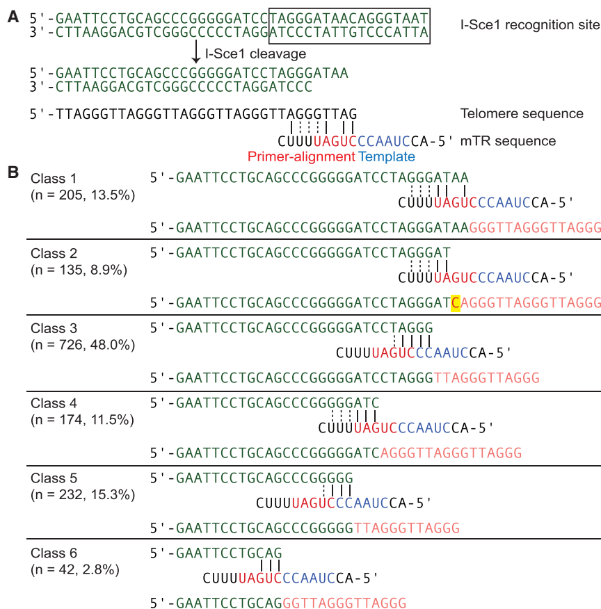
Figure 2. Classification of De Novo Telomere Addition
