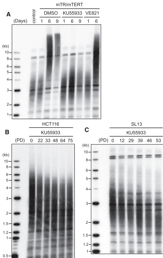
Figure 4. ATM Is Essential for Bulk Telomere Elongation in Both Human and Mouse Cells
