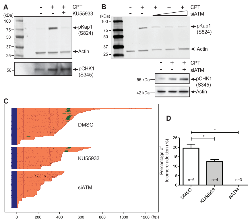
Figure 3. ATM Kinase Is Required for Telomere Addition
