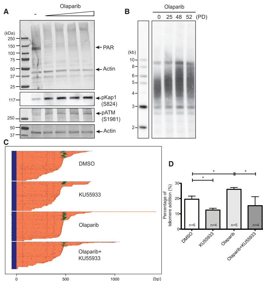
Figure 5. Activation of ATM Kinase Pathway Elongates Telomeres
