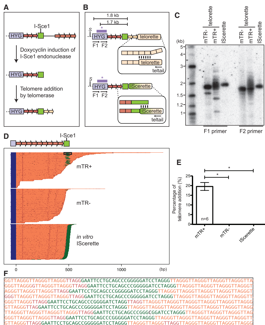
Figure 1. De Novo Telomere Addition Occurs Only in Telomerase-Positive Cells
