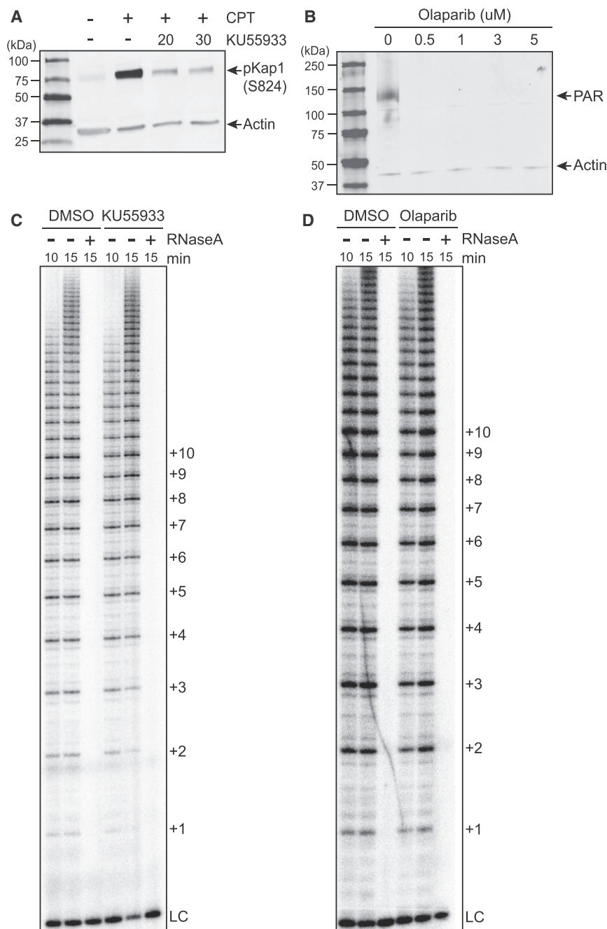
Figure 6. Telomerase Activity Is Unaffected by Either Olaparib or KU55933 Treatment
