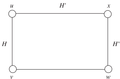
Fig. 1. A 4-cycle of R(B) .
