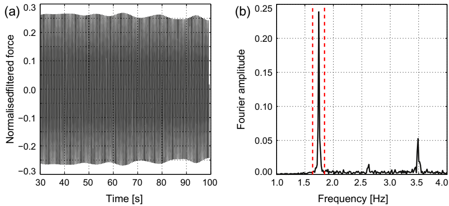
Fig. 14. (a) Time-domain of the narrow-band force component around the first harmonic. (b) Fourier spectrum of the force (normalised to body weight). Dashed lines represent filter bandwidth.
