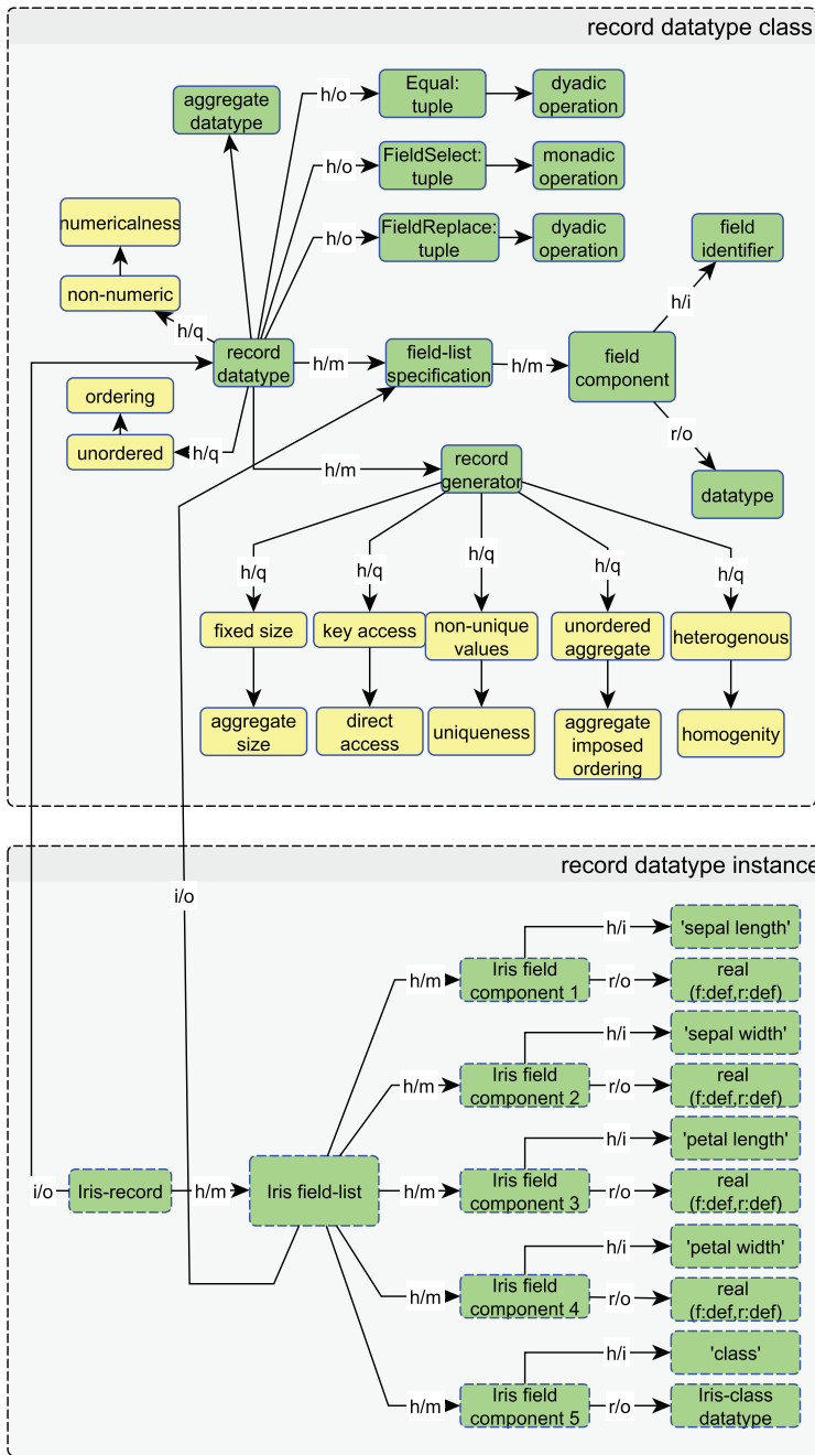
(a) Record datatype class and instance
