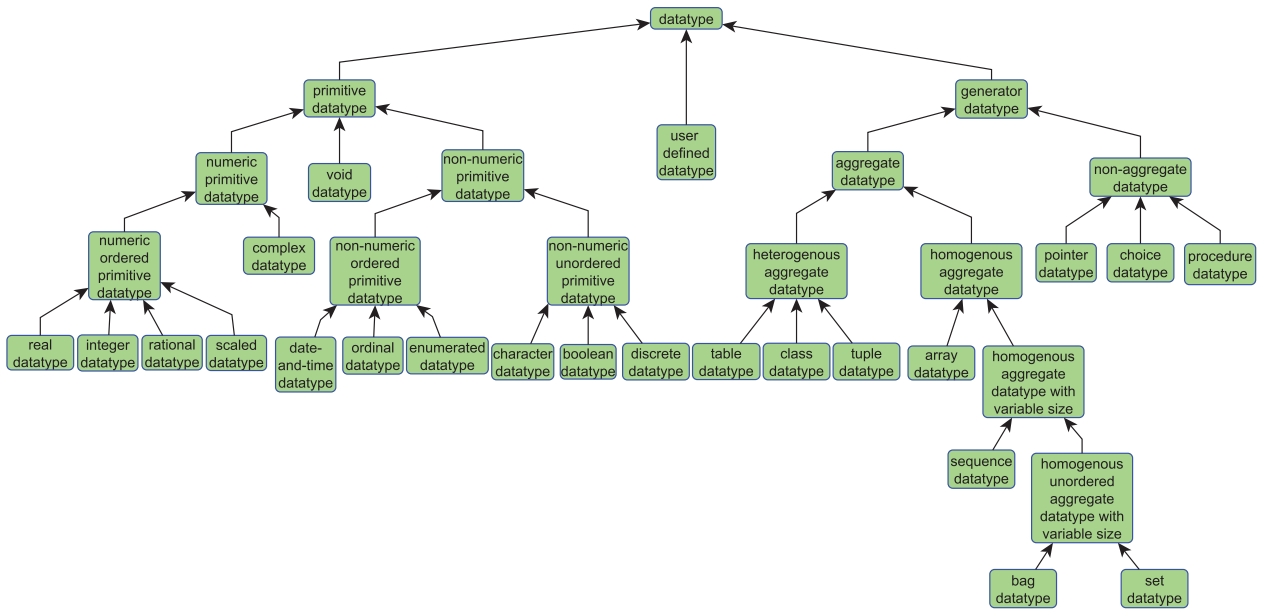
Fig. 3. The OntoDT datatype taxonomy. The rectangular boxes represent ontology classes. Unlabeled arrows represent is-A relations.
