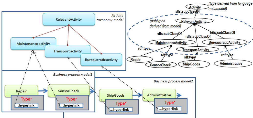
Fig. 9. Merging customizable model-level types with metamodel's prescribed types
