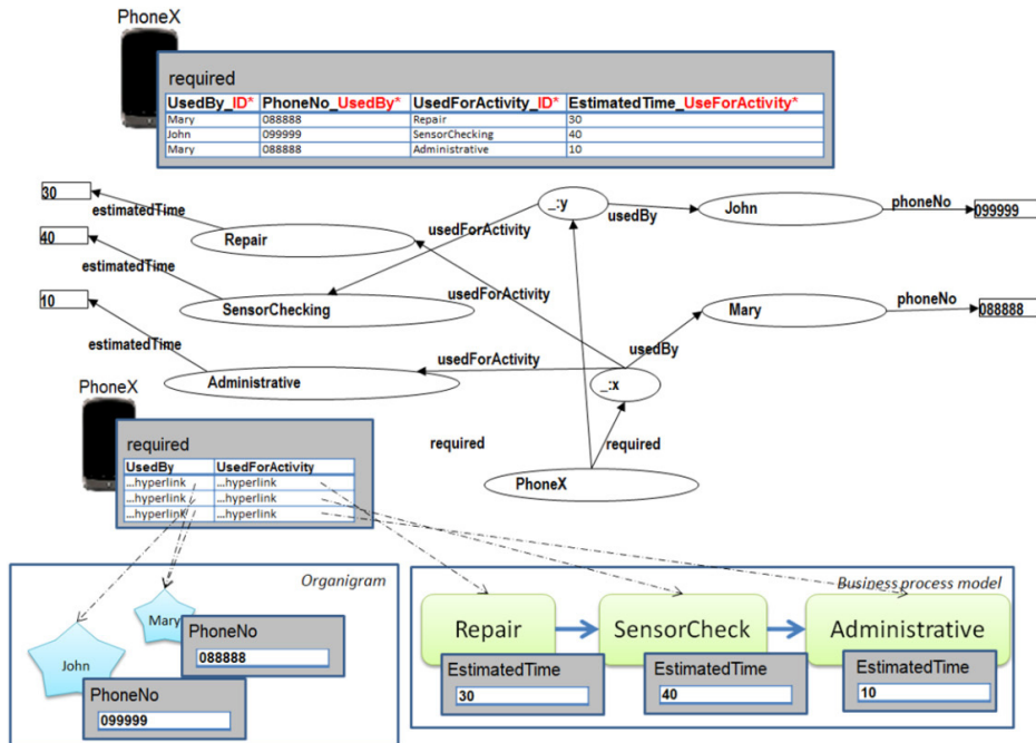
Fig. 7. Defusing the normalization anti-pattern
