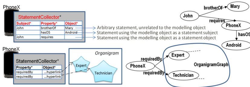
Fig. 4. The statement collector pattern
