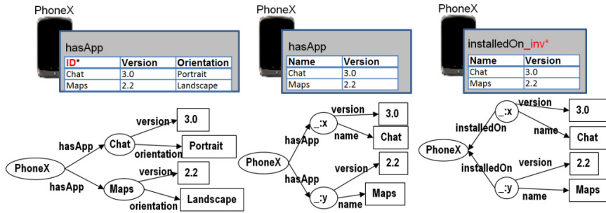
Fig. 5. The non-canvas object pattern
