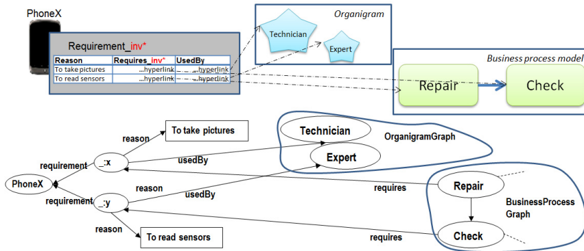
Fig. 6. The n-ary relation pattern
