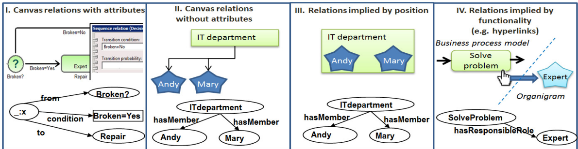
Fig. 3. Modeling relation patterns and their corresponding graph data structures
