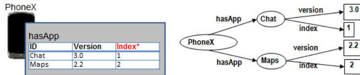
Fig. 8. Ordered variant of the non-canvas object pattern
