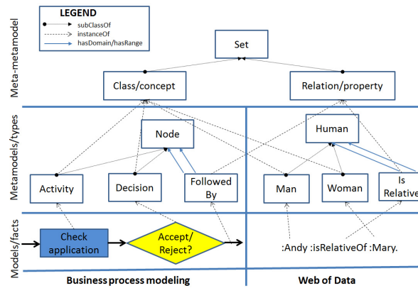
Fig. 1. A convergence between diagrammatic modeling and Web of Data across abstraction layers
