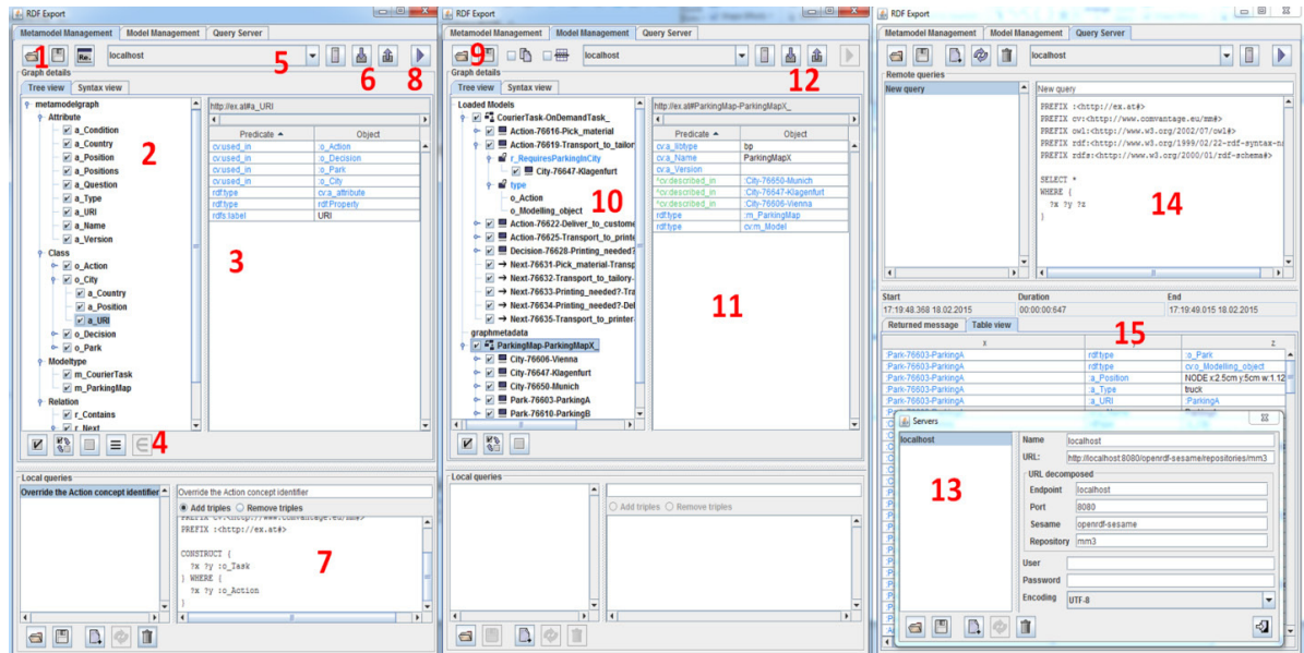
Fig. 10. Screenshots of the model-to-Linked Data converter prototype
