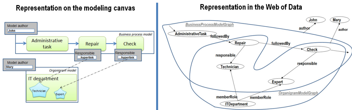
Fig. 2. Generated graph structure for inter-linked diagrams
