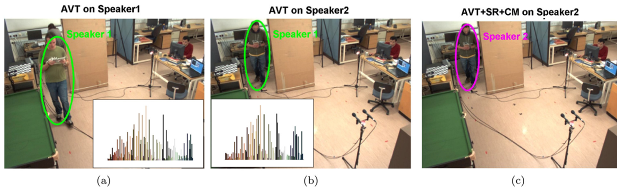
Fig. 9. ‘Abandoning’ tracking results. (a) Shows the AVT locked onto Speaker1 . In (b) the other person appears while Speaker1 has left the scene. The ID assessed by the AVT is still Speaker1 meaning the AVT cannot make a distinction between IDs. In fact, the video tracker features for the two people, i.e., the histogram of colours at the bottom of (a, b), are very similar. In (c) instead, the AVT+SR+CM solution correctly the person ID is Speaker2 . (For interpretation of the references to color in this figure caption, the reader is referred to the web version of this paper.)
