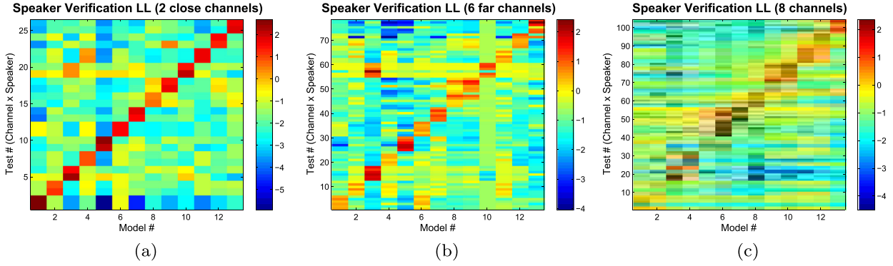
Fig. 3. The speaker verification confusion matrix for close and far microphone setups. The speaker verification confusion matrix for close and far microphone setups. This figure shows the ability of the implemented SR unit to verify ID of people in the recorded pool of voices for (a) 2 close microphones (1 close field microphone pair); (b) 6 far microphones (3 far field microphone pairs); and (c) the total 8 channels (4 microphone pairs: 1 in the close field plus 3 in the far field). Results show that the best performance is obtained for close distance recording, i.e., (a), whereas in (b) and (c) speaker recognition is severely compromised due to the 3 pairs of far distance microphones.
