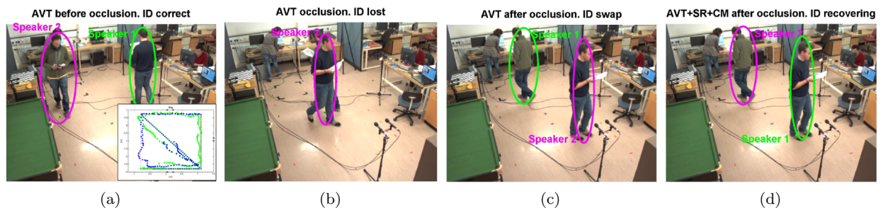
Fig. 10. ‘Crossing’ tracking results. In (a) the AVT correctly identifies both people ID. In (b) a short term occlusion leads track to merge. This results in (c) in an ID swap as the ellipses colors have exchanged. On the other hand (d) presents the AVT+SR+CM result for the same situation, i.e., correct ID recovering after the occlusion. (For interpretation of the references to color in this figure caption, the reader is referred to the web version of this paper.)
