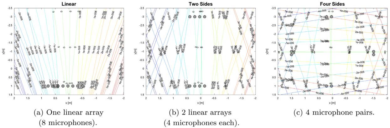
Fig. 6. Isolines, i.e., hyperbolas loci. An isoline indicates all points of a constant difference in distance from two points. 2D contour maps in the xy plane when z=1.7 m for the (a) linear array of microphones, (b) 2 linear arrays of 4 microphones on two sides of the room, (c) 4 pairs of microphones of the 4 sides of the room. The last, has the more dense number of intersecting isolines, i.e., a higher number of possible solutions.
