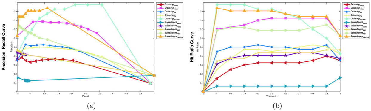
Fig. 13. Comparison to baseline method (BM) [17]. Precision–recall and hit ratio curves for the testing videos averaged over the total number of frames. Results of the proposed method (PM) are compared first against audio and video only results, then against the baseline method (BM) of [17]. Besides, the proposed method aided by the information about the speaker ID, i.e., PM+SR is given, showing that the method is actually suitable for diarisation purposes in cross-talking scenarios whenever a record of the speaker ID over time is kept.
