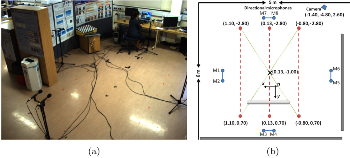
Fig. 5. In (a) a picture of the room used for our set of experiments is shown. (b) illustrates its layout and sensor setups.
