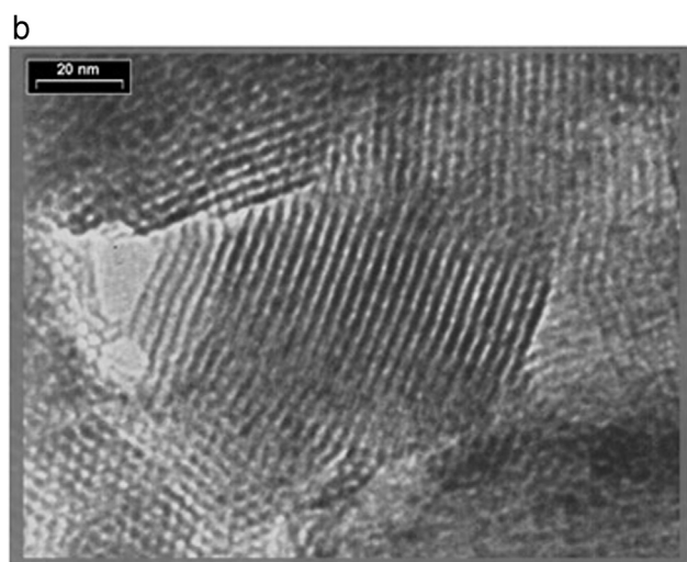
Fig. 3. TEM image of Si-MCM-41 silica (Me 3 ), b) cells alongside the pore of mesoporous MCM-41 (Me 3 ).
