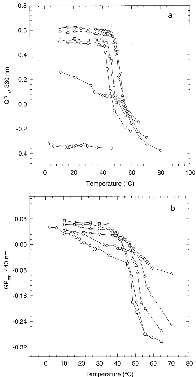
Fig. 2. GP_{ex} (a) and GP_{em} (b) values as a function of temperature for Laurdan in aggregates of: DPPC (○); DPPC/Gg 4 Cer mixtures at 6 (□), 36.4 (△), 69.7 (▽) mol% of Gg 4 Cer; Gg 4 Cer (◇) and G M1 (○). The GP_{ex} values were calculated using an excitation wavelength of 360 nm. The GP_{em} values were calculated using an emission wavelength of 440 nm. The main phase transition temperatures were calculated from the dGP/dT and the values obtained were: pure DPPC = 41°C; DPPC/Gg 4 Cer mixtures at a mol% of Gg 4 Cer of: 6% = 42°C, 36.4% = 46°C and 69.7% = 52°C; pure Gg 4 Cer = 56°C. Buffer was 20 mM Tris-HCl-50 mM NaCl (pH 7.4). Laurdan concentration was 0.5 μM, lipid/probe ratio was 400:1.
