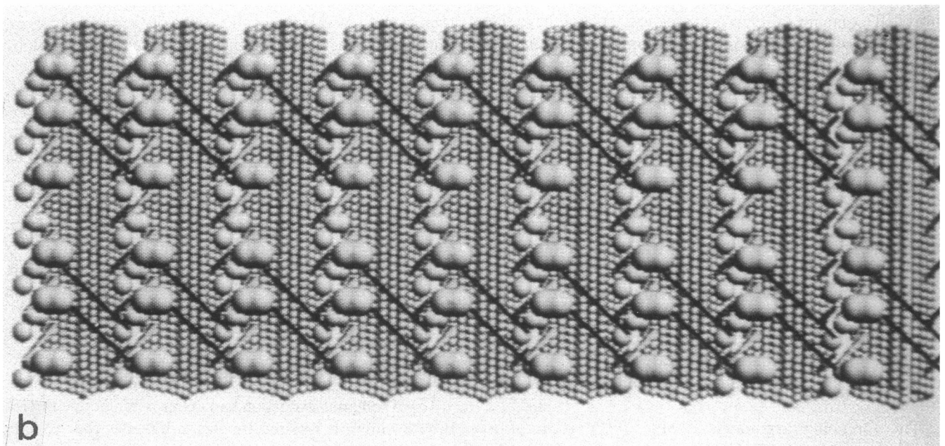
FIGURE 1 (a) Computer-generated model of complete axoneme, viewed to give an impression of the three-dimensional character of the structure. (b) Computer-generated model of the unrolled axoneme; the central complex has been omitted from the model.
