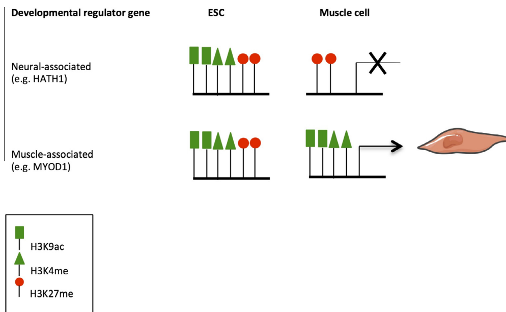
Fig. 1 Bivalent chromatin marks in ES cells and during differentiation to muscle cells.
