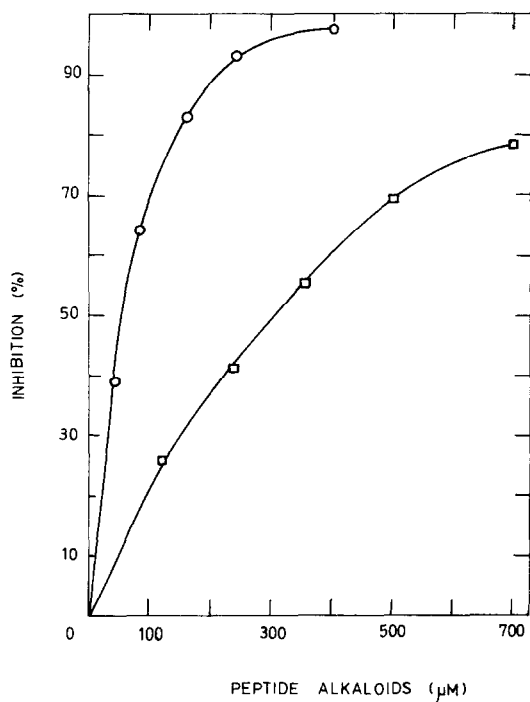
Fig. 1. Effect of discarines A and B on non-cyclic photophosphorylation in spinach chloroplasts. ATP synthesis in control tubes was 42 \mu\text{moles/mg} chlorophyll per hr. ( \circ-\circ-\circ ) Discaraine B; ( \square-\square-\square ) discaraine A.
