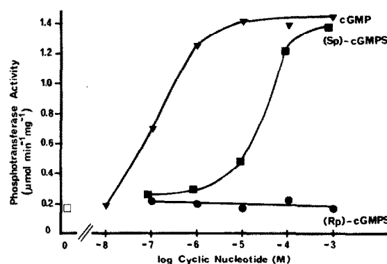
Fig. 2. Effects of cGMP ( \blacktriangledown ), (Sp)-cGMPS ( \blacksquare ), and (Rp)-cGMPS ( \bullet ) on the activity of cGMP-dependent protein kinase. The activity of the enzyme in the absence of cyclic nucleotides is indicated ( \square ). Similar data were obtained in several separate experiments.
