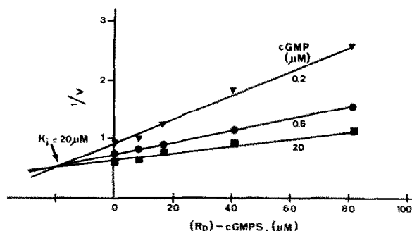
Fig. 3. Dixon plot demonstrating the competitive inhibition by (Rp)-cGMPS of the cGMP-induced activation of cGK. 1/V is the reciprocal value of the phosphotransferase activity ( \mu\text{mol} \cdot \text{min}^{-1} \cdot \text{mg}^{-1} ) measured. Similar results were obtained in three separate experiments.
