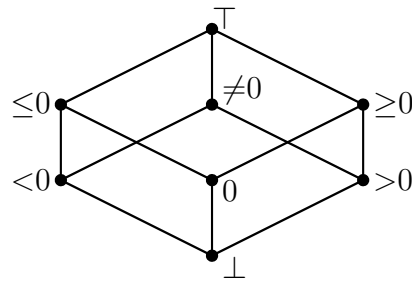
Fig. 1. Hasse diagram for the signs abstract domain for a single variable
