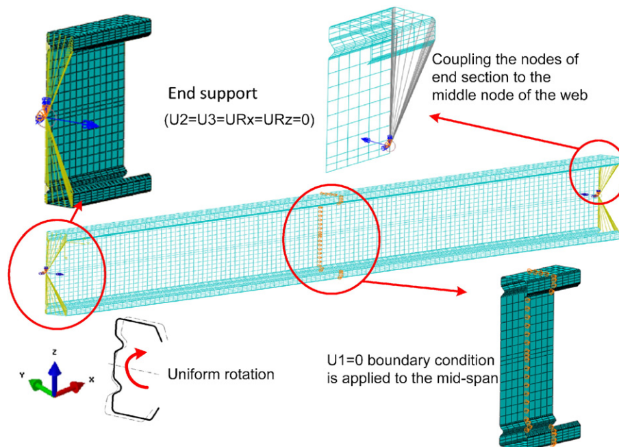
Fig. 19. Boundary conditions in the FE models of channel sections.
