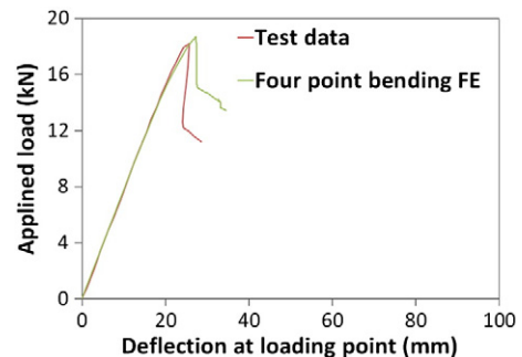
Fig. 14. Comparison between experimental results and FE analyses for laterally braced specimen D11.5Z092-3.
