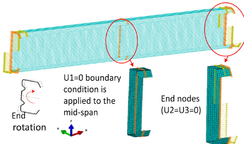
Fig. 21. FE model for laterally unbraced standard and optimise beams.
