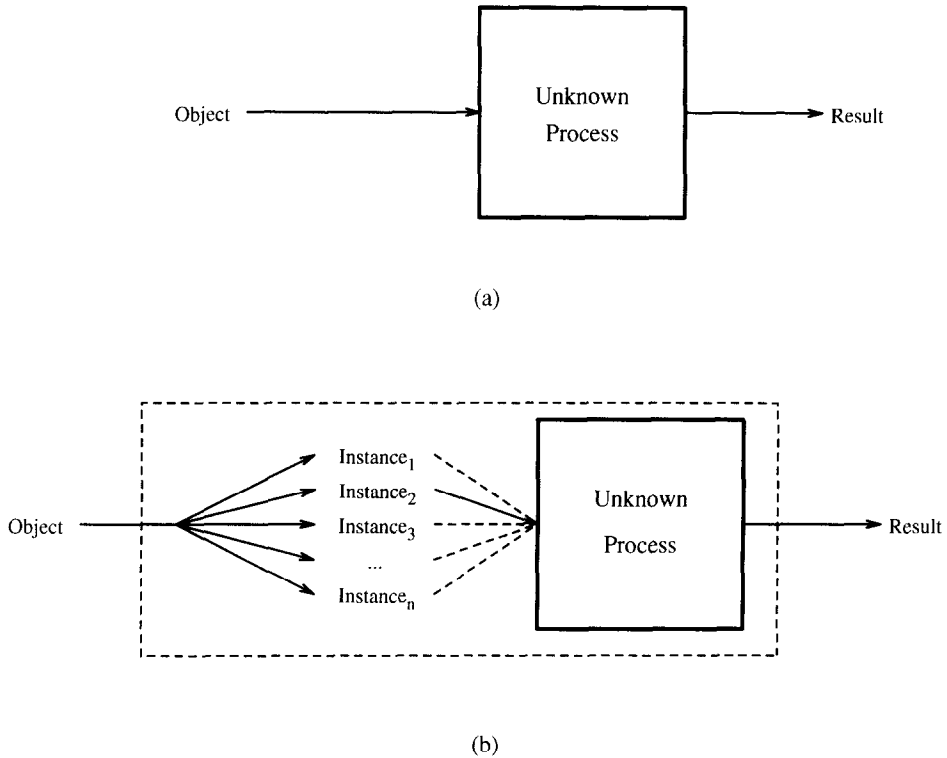
Fig. 1. Supervised learning: (a) usual situation and (b) multiple instance situation.
