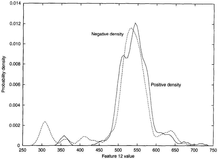
Fig. 9. Kernel density estimate for positive and negative feature vectors along feature 12 in musk data set 1.
