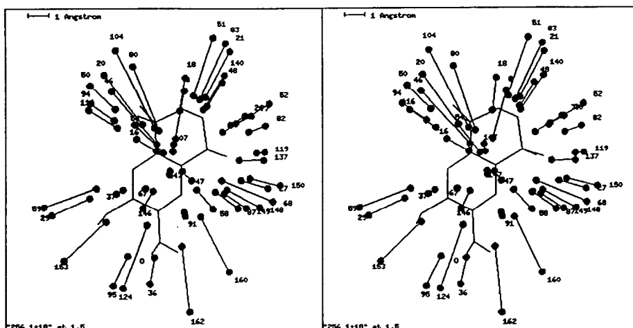
Fig. 24. The musk data set 2 APR and a structure diagram (bond graph) for conformation 18 of molecule "256". All APR bounds are shown in this single stereo pair. The oxygen atom is at the bottom on the image.
