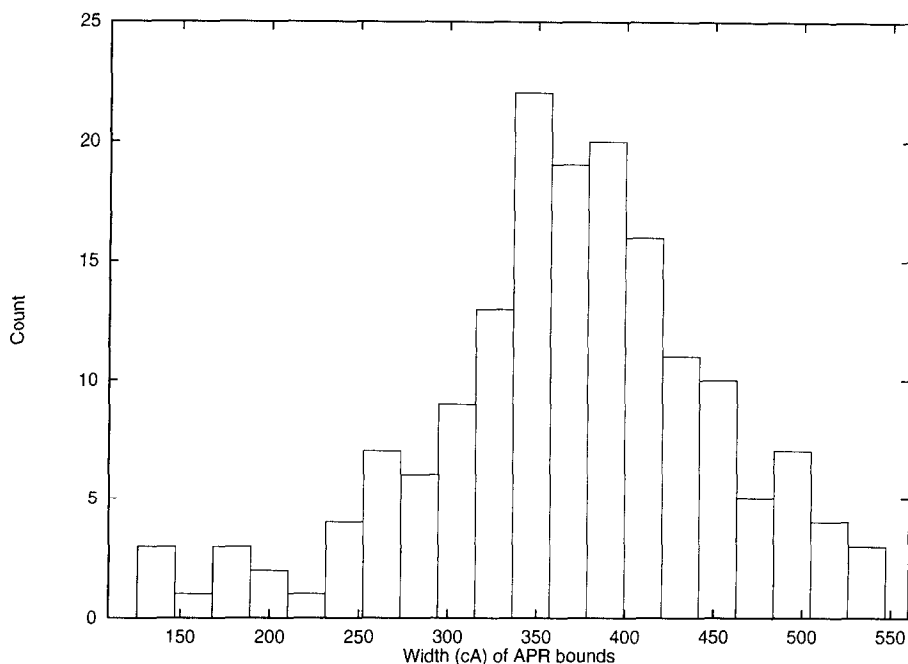
Fig. 6. Histogram of the width of the bounds of an APR that tightly contains all feature vectors in musk data set 1.
