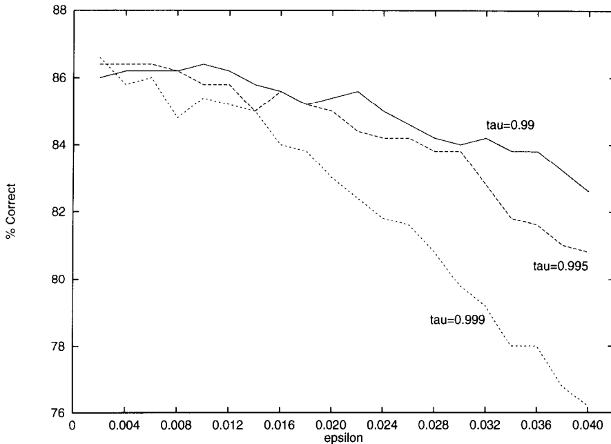
Fig. 19. Performance of iterated discrimination on the artificial data set as a function of its parameters \epsilon and \tau .
