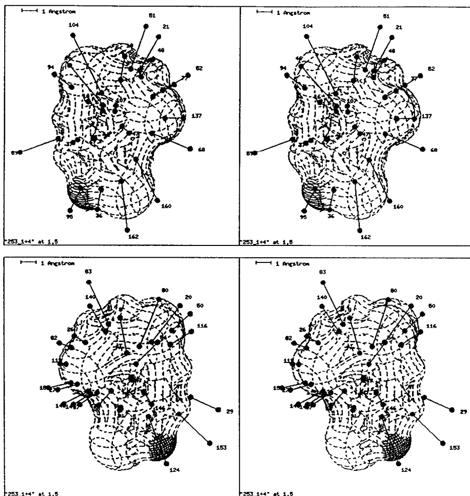
Fig. 23. The musk data set 2 APR binding hypothesis applied to classify conformation 4 of molecule "253" (a non-musk). The upper two frames give a "front view"; the lower two frames give a "back view" of the same molecule. Note that bounds 59 (in the "front view") and 29 (in the "back view") are violated.
