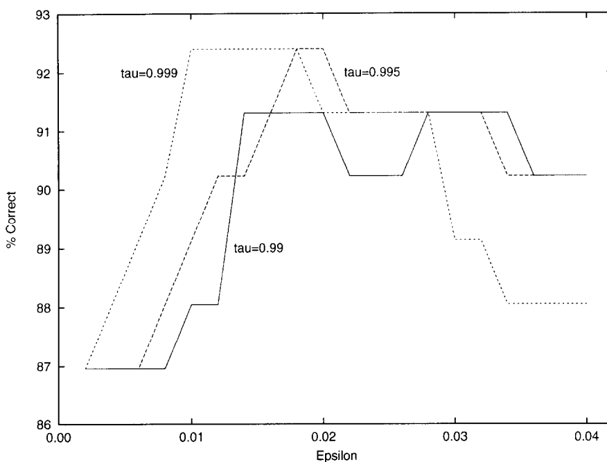
Fig. 20. Performance of iterated discrimination on musk data set 1 as a function of \tau and \epsilon .
