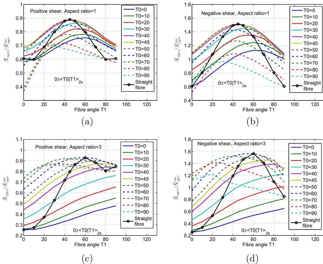
Fig. 4. Square VAT plate 0 \pm (T_0|T_1)_{2s} subjected to in-plane shear load (a) positive shear, aspect ratio = 1 (b) negative shear, aspect ratio = 1 (c) positive shear, aspect ratio = 3 (d) negative shear, aspect ratio = 3.
