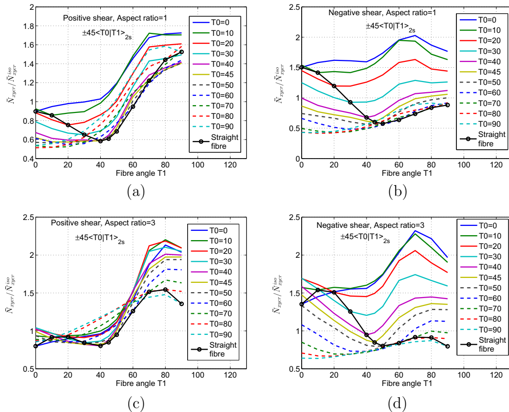
Fig. 13. Square VAT plate \pm 45\langle T_0|T_1 \rangle_{2s} subjected to in-plane shear displacement (a) positive shear, aspect ratio = 1 (b) negative shear, aspect ratio = 1 (c) positive shear, aspect ratio = 3 (d) negative shear, aspect ratio = 3.
