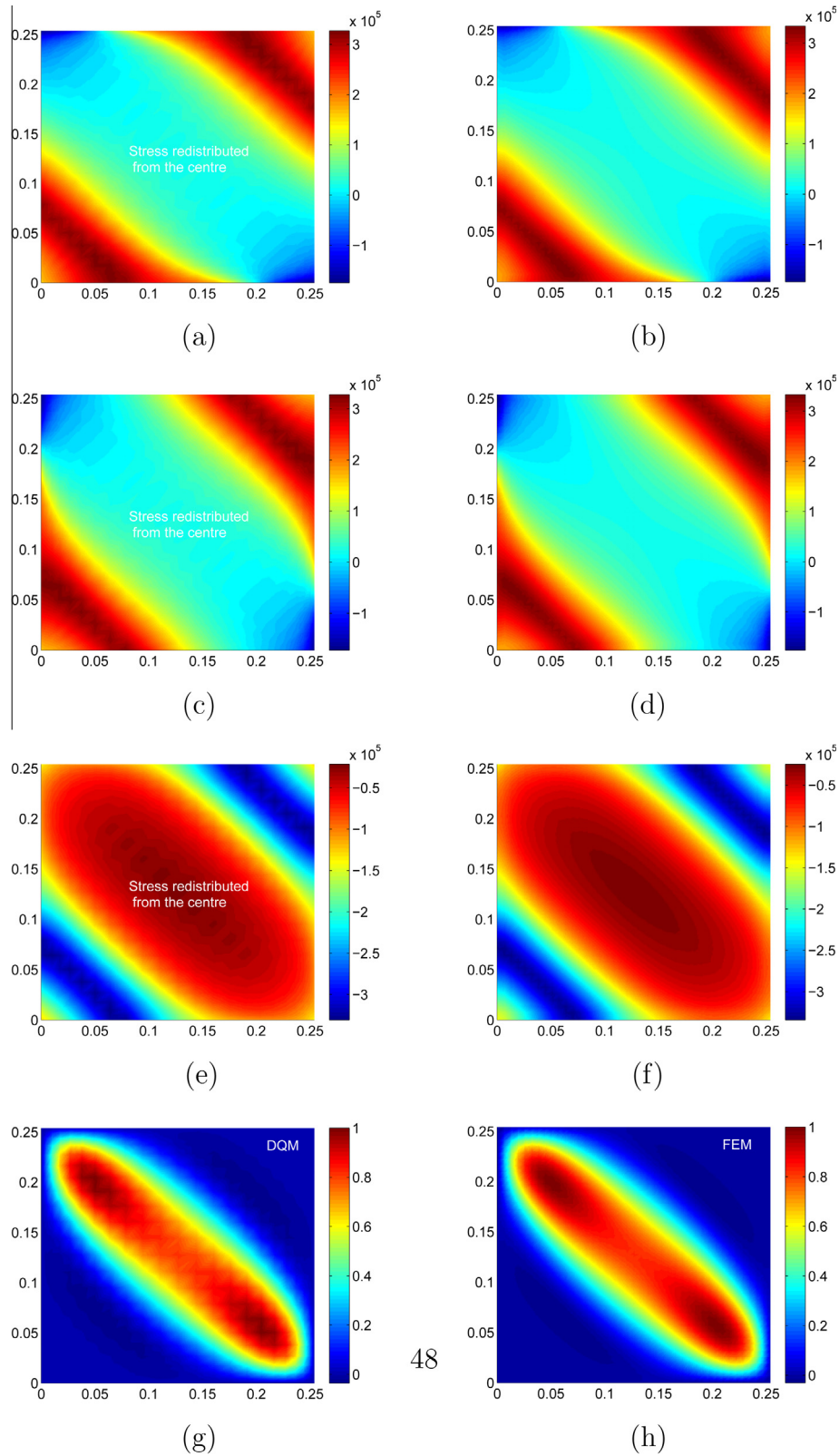
Fig. 15. Square VAT plate [45 \pm (30/80)]_{2z} , subjected to in-plane negative shear displacement: stress resultant distribution \bar{N}_x (a) DQM (b) FEM, stress resultant distribution \bar{N}_y (c) DQM (d) FEM, stress resultant distribution \bar{N}_{xy} (e) DQM (f) FEM, buckling mode shape (g) DQM (h) FEM.
