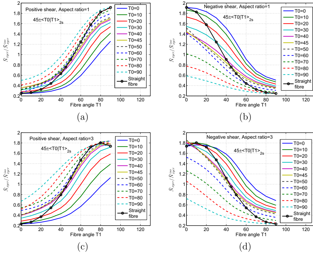
Fig. 5. Square VAT plate 45 \pm \langle T_0|T_1 \rangle_{2s} subjected to in-plane shear load (a) positive shear, aspect ratio = 1 (b) negative shear, aspect ratio = 1 (c) positive shear, aspect ratio = 3 (d) negative shear, aspect ratio = 3.
