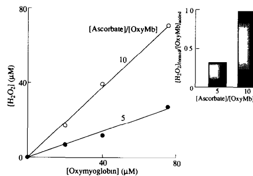
Fig. 3. H_2O_2 formation during the reaction of ascorbate and oxymyoglobin. Assay conditions: different amounts of oxymyoglobin (10–80 \mu M) in helium-purged 0.1 M potassium phosphate buffer, pH 5.5, were supplemented with ascorbic acid (to reach a [ascorbic acid]/[myoglobin] ratio of 5 or 10). Insert: [H_2O_2]_{formed}/[OxyMb]_{added} ratio vs. [ascorbic acid]/[oxymyoglobin]. Abbreviation: oxyMb, oxymyoglobin.
