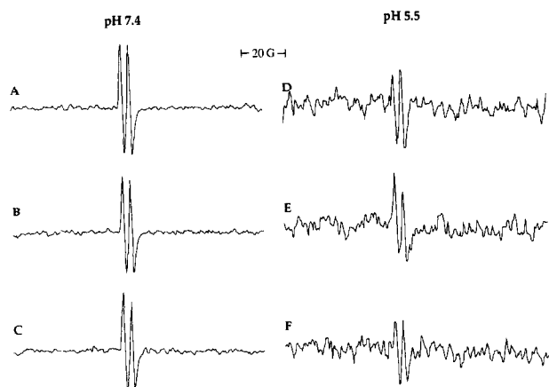
Fig. 2. Ascorbyl radical formation during the reaction of ascorbate with oxymyoglobin. Left panel: the reaction mixture consisted of 1 mM ascorbic acid in 0.1 M potassium phosphate buffer, pH 7.4, supplemented with 0.2 mM oxymyoglobin. (A) No additions; (B) plus 1 \mu M superoxide dismutase; (C) plus 500 U \cdot ml ^{-1} catalase. Right panel: as above at pH 5.5. Instrument settings as described in section 2. Instrument scale: left panel, 19; right panel, 17.
