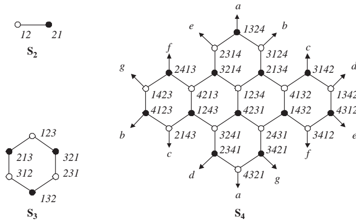
Fig. 5. The star graphs S_2 , S_3 , and S_4 .
