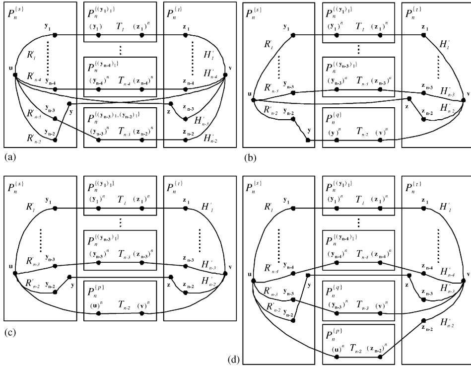
Fig. 4. Illustration for Theorem 2.
