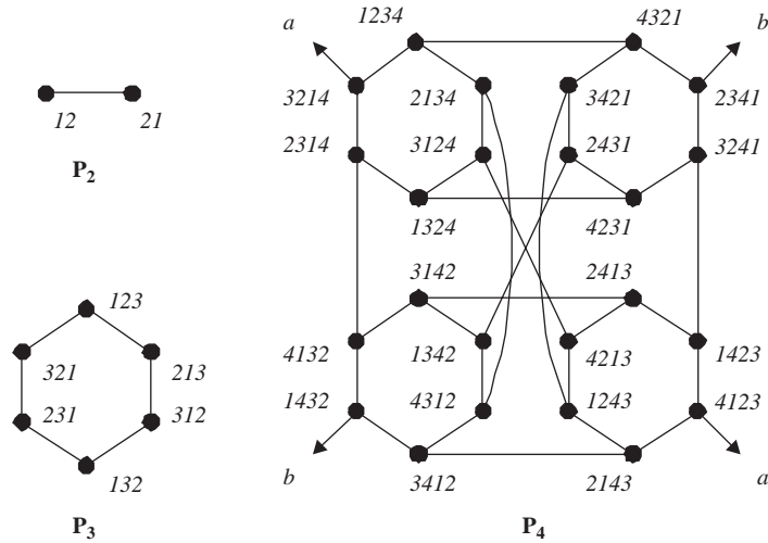
Fig. 1. The pancake graphs P_2 , P_3 , and P_4 .
