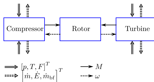
Fig. 11. A turbocharger model.
