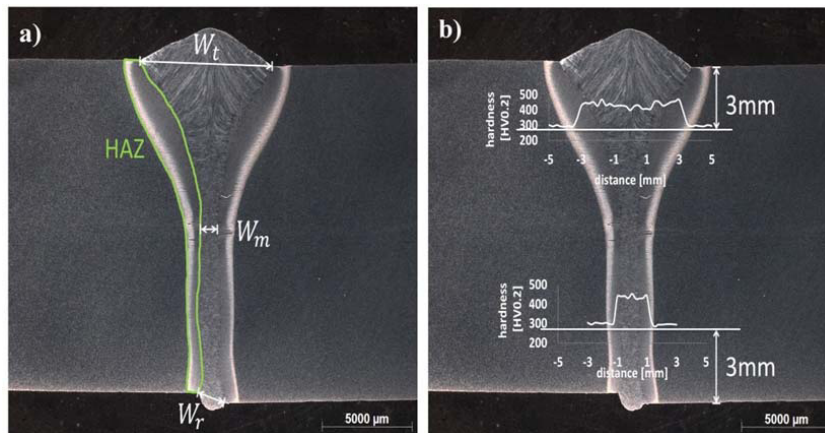
Fig. 3. (a) Determination of the geometric variables; (b) determined hardness profiles.
