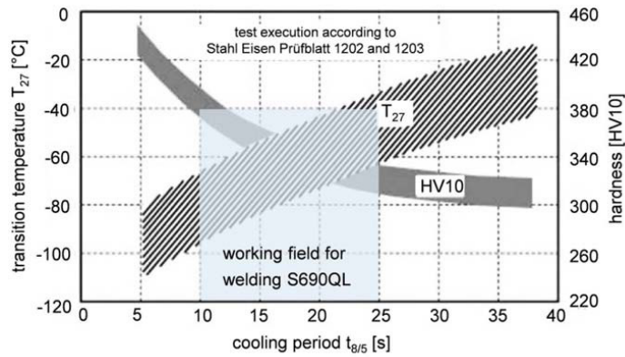
Fig. 1. Hardness and toughness of S690QL depending on the cooling period t_{8/5} ( Hamme et al. , 2000).
