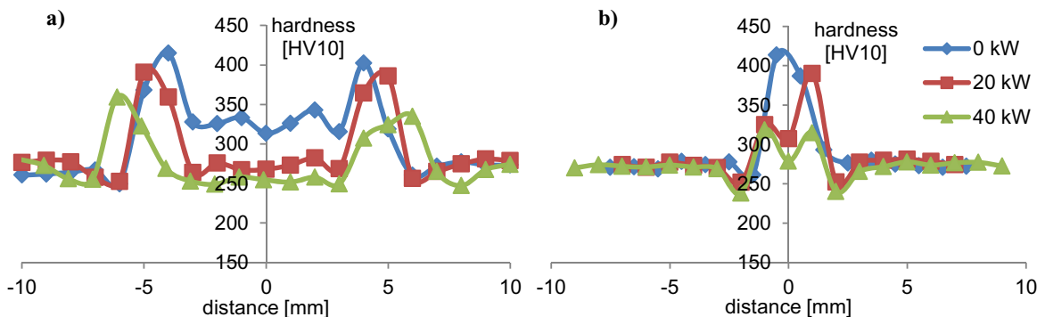
Fig. 8. Hardness distribution at the top (a) and at the root (b) of S690QL with a thickness of 20 mm.
