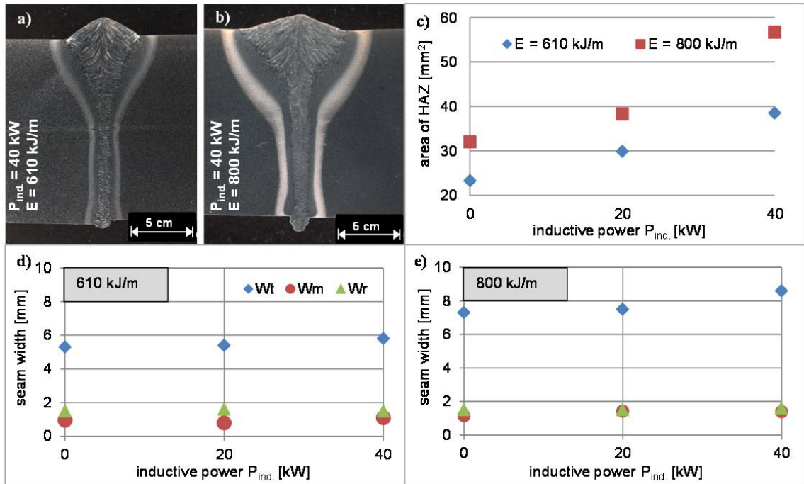
Fig. 5. Cross-sections (a-b) and results of the weld seam geometry and the HAZ (c) depending on the inductive power, and an energy per unit length of 610 kJ/m (d) and 800 kJ/m (e).
