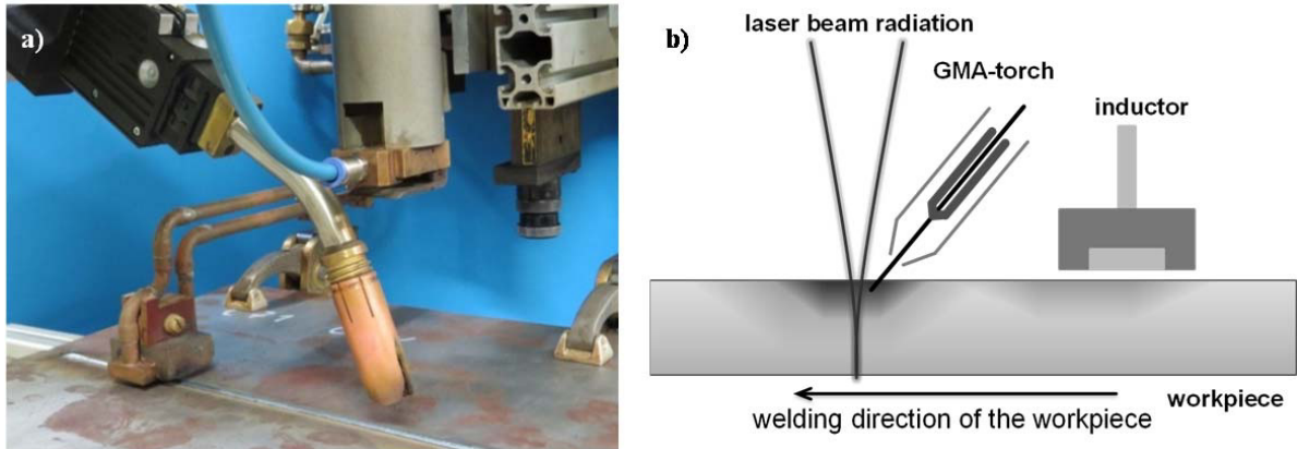
Fig. 2. Real (a) and schematic (b) experimental setup.
