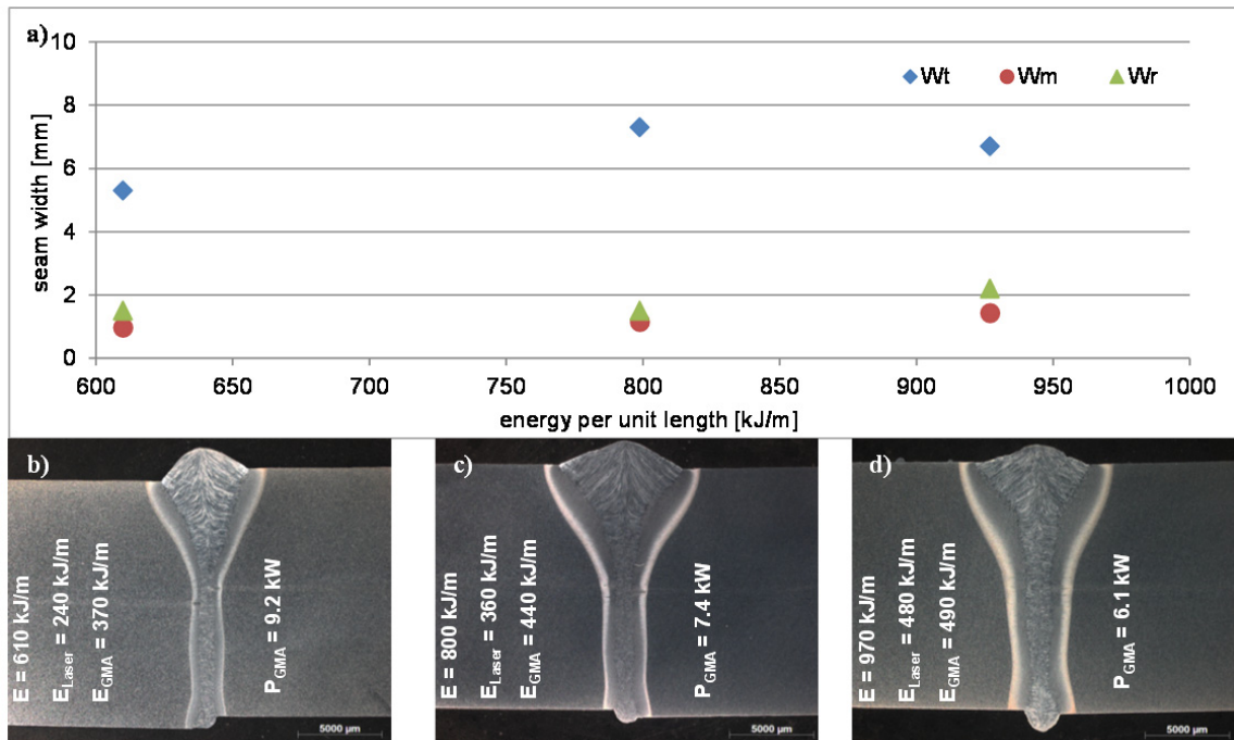
Fig. 4. Influence of the energy per unit length on the geometry of the welding seam, welded with b) 610 kJ/m, c) 800 kJ/m, d) 970 kJ/m.
