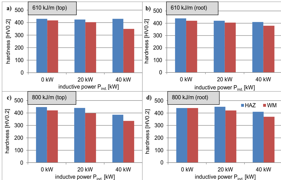
Fig. 6. Hardness of the weld metal and HAZ at the top and the root depending on the energy per unit length and the inductive power, (a) 610 kJ/m at the top, (b) 610 kJ/m at the root, (c) 800 kJ/m at the top and (d) 800 kJ/m at the root.
