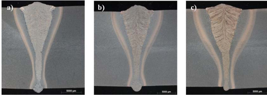
Fig. 7. Cross-sections of welding seam: P_{ind.} = 0 kW (a), 20 kW (b) and 40 kW (c).
