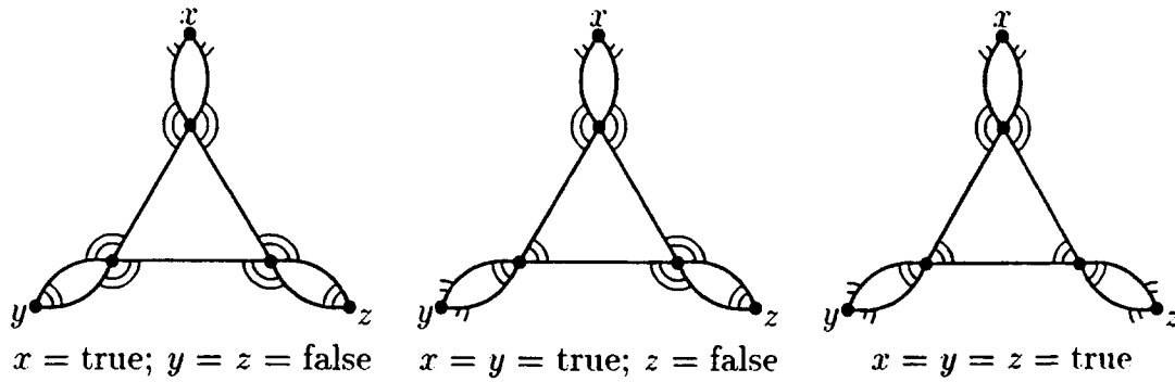
Fig. 7. Traversing a clause.
