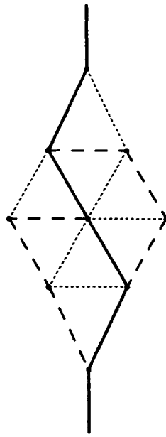
Fig. 8. Overlapping paths to the main cycle.
