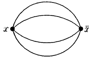
Fig. 5. Adjacent rim vertices.
