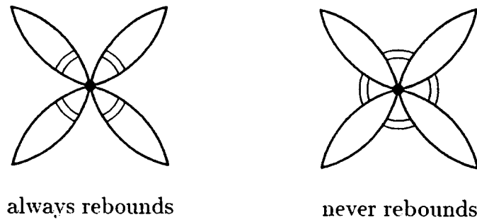
Fig. 4. Rebounding at wheel vertices.
