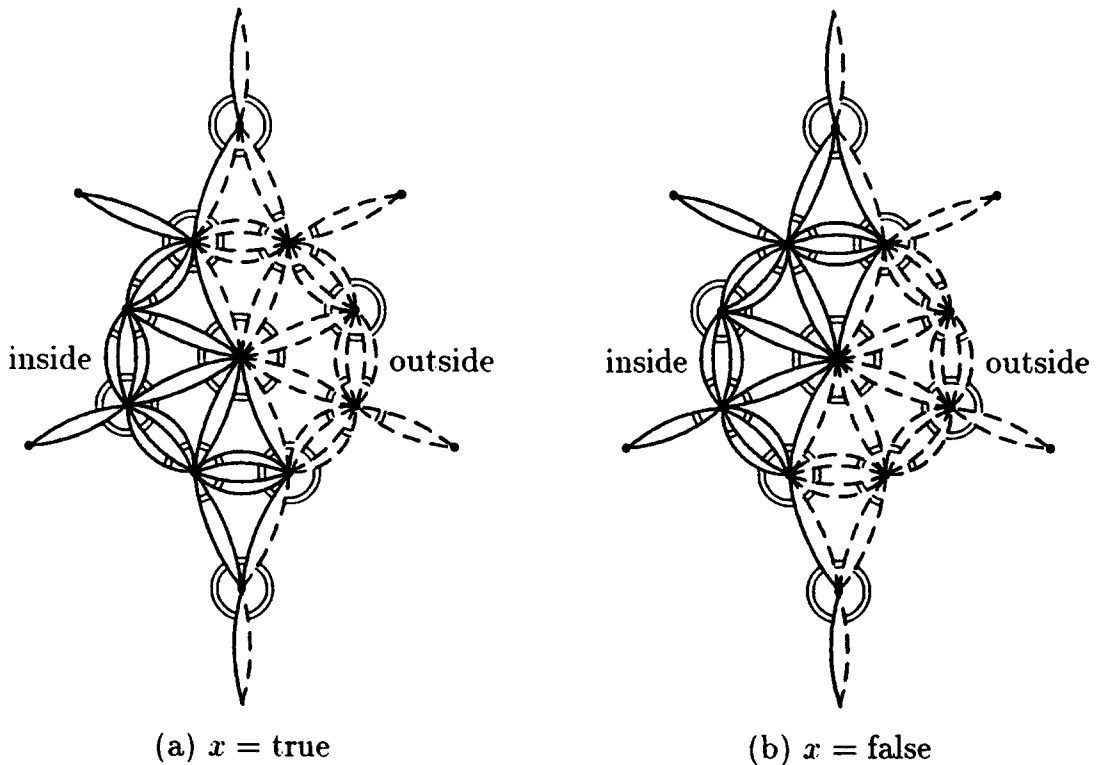
Fig. 6. Traversing a wheel.
