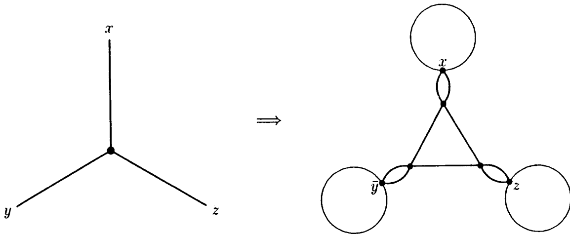
Fig. 2. Clause C = (x \vee \bar{y} \vee z) .
