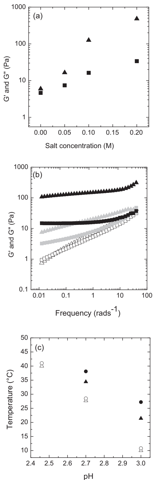
Fig. 5. Influence of NaCl concentration on acid pectin samples where the pectin concentration is 1%. (a) G' (triangles) and G'' (squares) at pH 3 at a strain of 0.5% and f=6.28 rad/s at T=5^\circ\text{C} . (b) Frequency dependency of samples containing different amount of NaCl from 0 M (open symbols), 0.05 M (gray symbols) to 0.1 M (black symbols) at T=5^\circ\text{C} . (c) Gelation (triangle) and melting (circle) temperatures in the absence of NaCl (open symbols) and in the presence of 0.05 M NaCl (solid symbols) at various pH.
