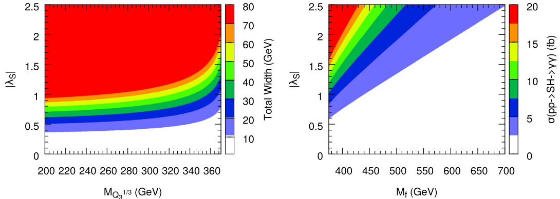
Fig. 4. Left Panel: The total decay width of the scalar S in the plane of adjoint fermion mass M_{Q_3^{\pm 1/3}} and universal Yukawa coupling |\lambda_S| for M_{Q_3^{\pm 1/3}} < M_S/2 . Right Panel: \sigma(pp \rightarrow \gamma\gamma) in the plane of heavy fermion masses and Yukawa coupling |\lambda_S| .
