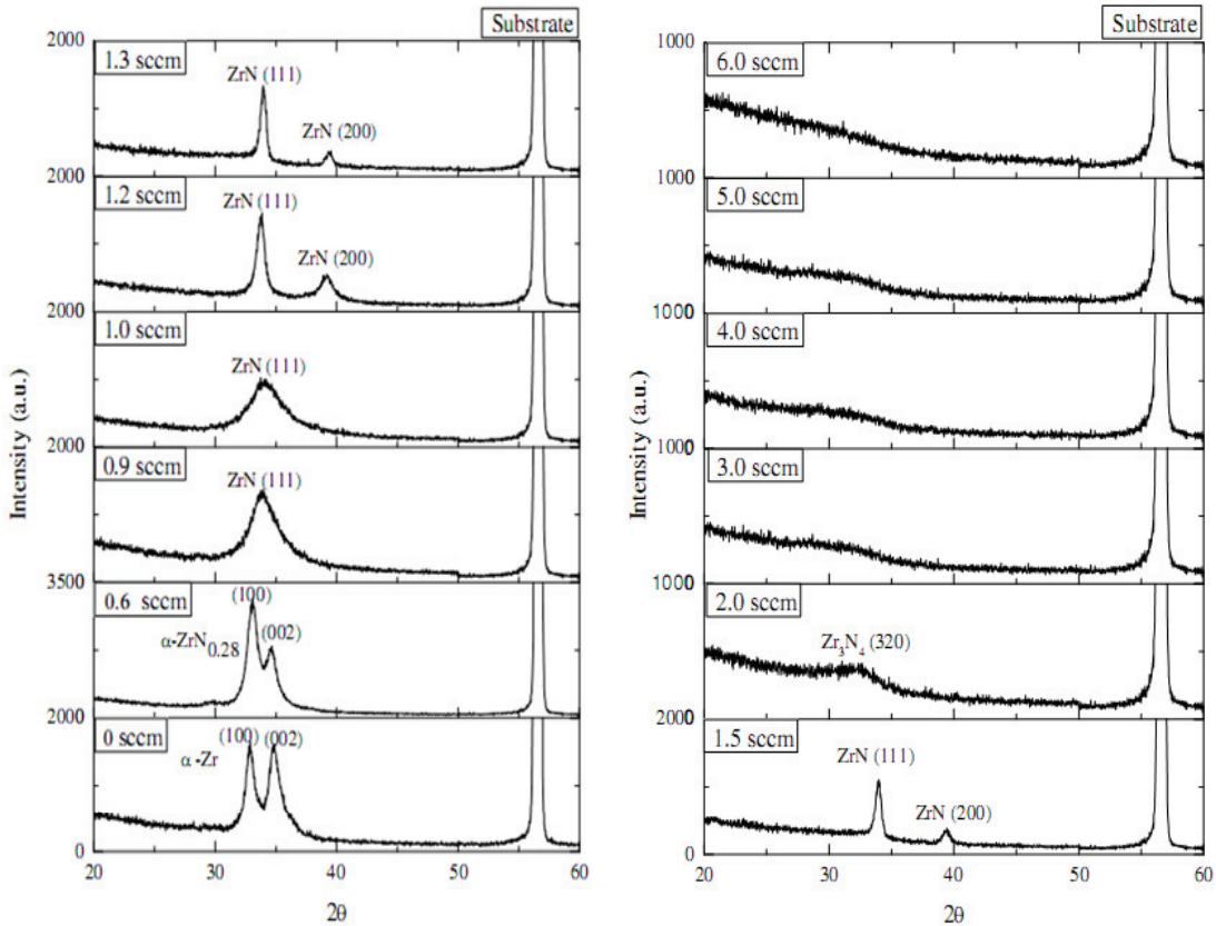
Fig. 3. X-ray diffraction patterns for Zr-N films deposited with various N 2 flow rates at Zr current of 0.6 A and deposition time of 15 minutes
