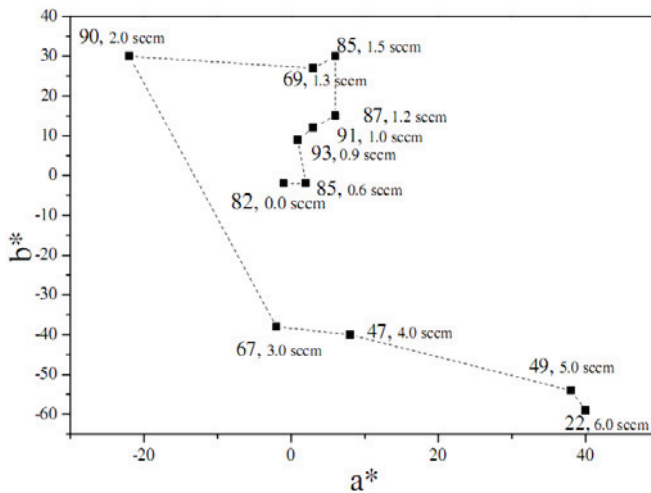
Fig. 2. Color of the zirconium nitride films in CIE L*a*b* color index in two dimensions of zirconium nitride film system. The given numbers of each point represent the value of lightness (L*) and N 2 gas flow rate
