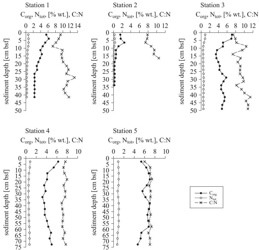
Figure 4. Organic carbon, total nitrogen and C:N ratio in the sediment profiles from the five coring stations
