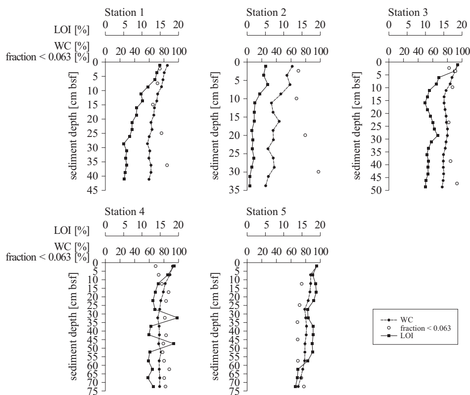
Figure 3. Water content, loss on ignition and the percentage of the < 0.063 mm fraction in the sediment profiles from the five coring stations
