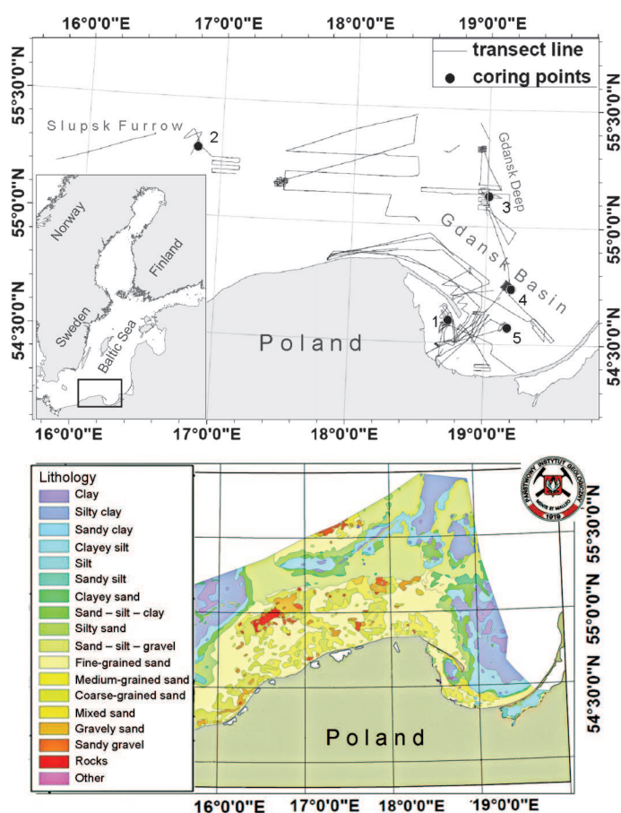
Figure 1. Map of the study area with acoustic and seismo-acoustic transects and coring points (black dots) (upper) and sedimentary units (lower) (map taken from Geochemistry of Baltic Sea Surface Sediments , Polish Geological Institute – National Research Institute, Warsaw 2011, S. Uścińowicz (ed.))
