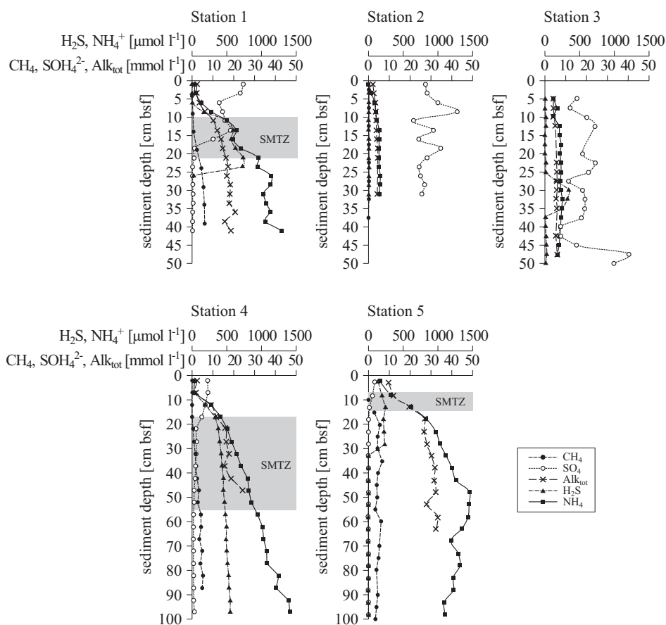
Figure 7. Concentrations of methane, sulphates, hydrogen sulphide, ammonium and total alkalinity in the sediment profiles at the five coring stations; the sulphate-methane transition zone SMTZ is marked in grey
