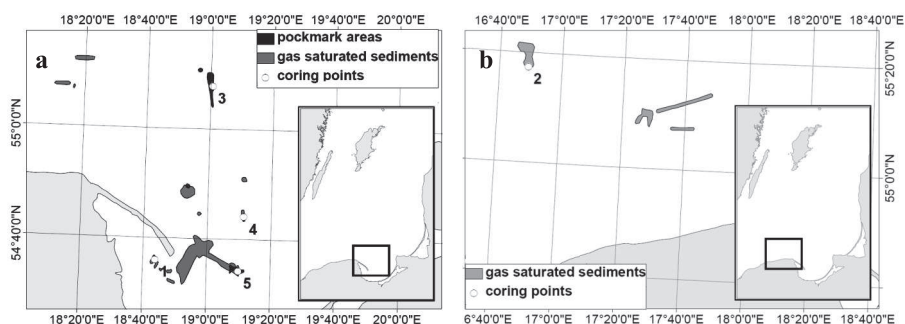
Figure 2. Areas with gas-saturated sediments and pockmarks in the Polish sector of the southern Baltic Sea: a) western part of the Gdańsk Basin and Gdańsk Deep, b) Słupsk Furrow and Słupsk Bank
