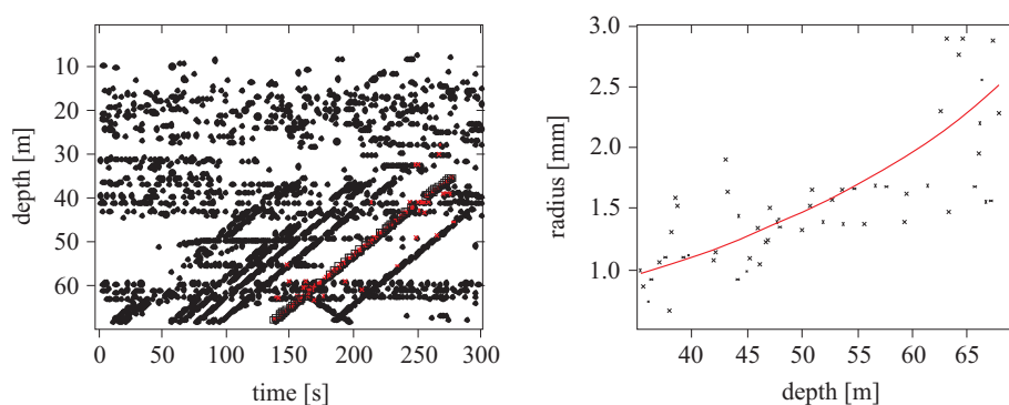
Figure 6. Images of traces of rising bubbles (red dots on the left) in the pockmark area as in Figure 5d, and radius changes with depth of a single bubble calculated on the basis of the measured instantaneous backscattering cross section (right)
