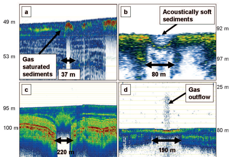
Figure 5. Different forms of shallow gas occurrence: gas pocket structures (a), buried pockmark (b), elongated pockmark or channel (c), active pockmark with a gas outflow (d). These forms were imaged with a 12 kHz ODOM III echosounder (a, c and d) and with a broadband chirp echosounder 40–80 kHz (b)
