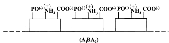
Fig. 11. Model III of the bilayer lipid surface, which presents the equilibria between the H^+ and OH^- ions from the solution and the species containing A_1BA_2 groups.
