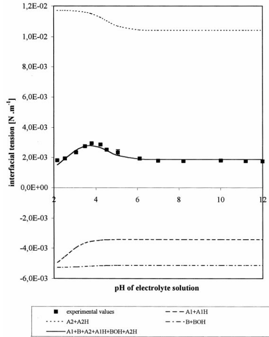
Fig. 9. The participation of the A 1 , B and A 2 groups, calculated for Model I, in dissociated and associated forms in the interfacial tension of the bilayer formed from PS, as a function of pH of the electrolyte solution.
