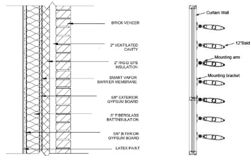
Fig. 5. (a) Improved facade system for the opaque exterior walls; (b) Curtain wall and shading system.
