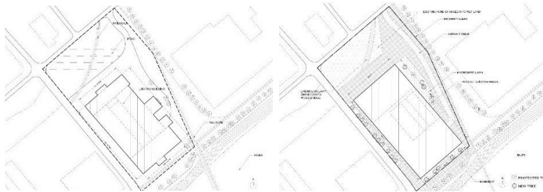
Fig. 3. (a) Site plan of existing building; (b) Site plan after retrofit.
