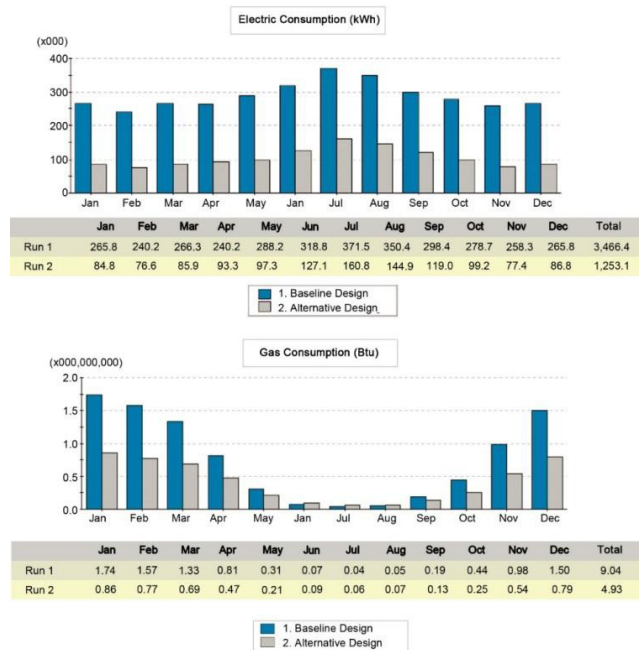
Fig. 7. Results of energy modeling (annual electricity and gas consumption) simulations.
