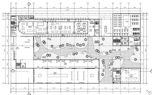
Fig. 4. First floor plan after retrofit, showing interior courtyard.
