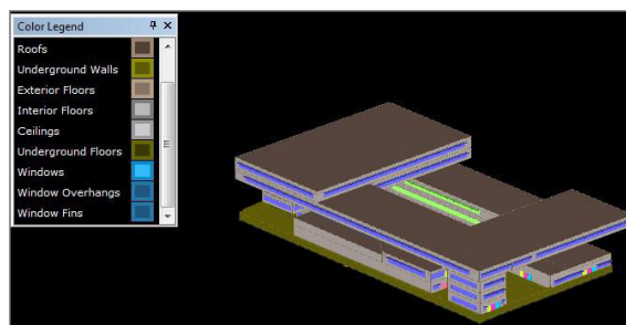
Fig. 6. Energy model in eQuest.
