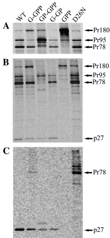
Fig. 2. Synthesis and processing of the wild-type and mutant polyprotein precursors. COS-1 cells transfected with wild-type or mutant proviruses were metabolically labeled 24 h post-transfection with [ 35 S]methionine-cysteine for 15 min and chased for 4 h. Intracellular proteins after the pulse (A) and chase (B) periods, as well as virus-associated proteins after the chase period (C) were immunoprecipitated using polyclonal anti-p27 (M-PMV CA) serum. The Gag-related polyprotein precursors and their major cleavage product the capsid protein are indicated: Pr180, Gag-Pro-Pol; Pr95, Gag-Pro; Pr78, Gag; p27, CA. D26N indicates a protease active site mutation in an otherwise the wild-type background.
