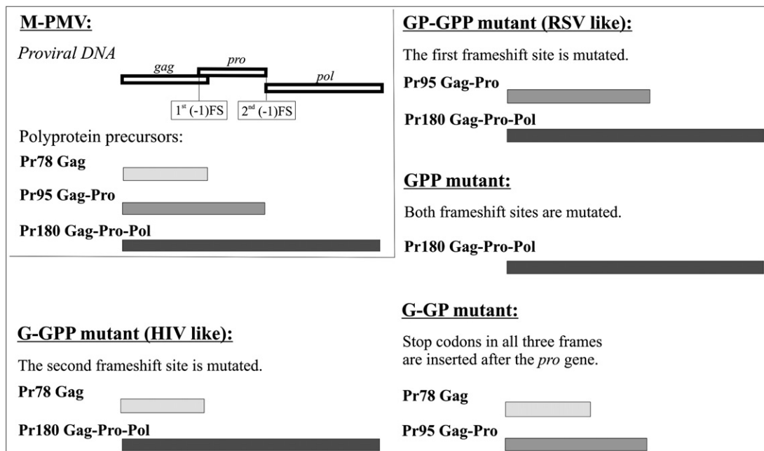
Fig. 1. Organization of the M-PMV gag , pro , and pol genes (upper left corner) and M-PMV frameshift mutants. The open boxes represent open reading frames in the proviral DNA; the filled boxes indicate the corresponding polyprotein precursors. (-1) FS indicates the frameshift site.
