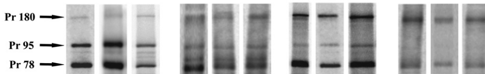
Fig. 5. Comparison of the wild-type and G-GPP mutant precursor ratios in pulse-labeled cells and in isolated immature capsids. COS-1 cells were metabolically labeled 24 h post-transfection with [ 35 S]methionine-cysteine. Cell lysates and immature particles isolated from cell lysates of pulse-labeled cells were immunoprecipitated using polyclonal anti-p27 (M-PMV CA) serum and the viral proteins were analyzed by phosphorimager. Three independent experiments were performed and are shown in the gels below the table under the corresponding data column. Table data give the average with the standard deviation. The Pr78, Pr95 and Pr180 polyproteins contain 5, 13 and 27 methionines, respectively.
