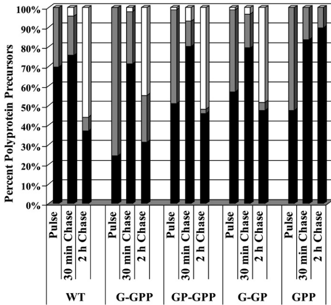
Fig. 4. The assembly of intracytoplasmic particles. COS-1 cells transfected with the wild-type and mutant genomes were metabolically labeled 24 h post-transfection with [ 35 S] methionine-cysteine for 15 min and chased for 30 min and 2 h. The assembled polyprotein precursors were pelleted from cell lysates by centrifugation through a 20% (w/v) cushion. Viral proteins from the pellet, supernatant and culture medium were immunoprecipitated and quantified using ImageQuant software. The sum of intensities of all Gag-related polyproteins plus that of the capsid protein at each time point was regarded as 100%. Black- and grey- portions of bars indicate the percentage of intracellular Gag-related precursors present in the pellet and supernatant form the cell lysates, respectively. The amounts of released (extracellular) viral proteins represent the white portions of the bars.
