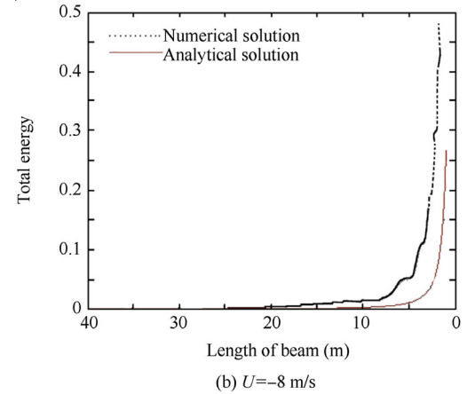
Fig. 10 Comparison between analytical solution and numerical solution for different retracting velocities.
