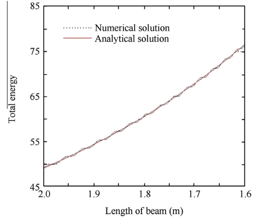
Fig. 9 Energy variation with length of beam.
