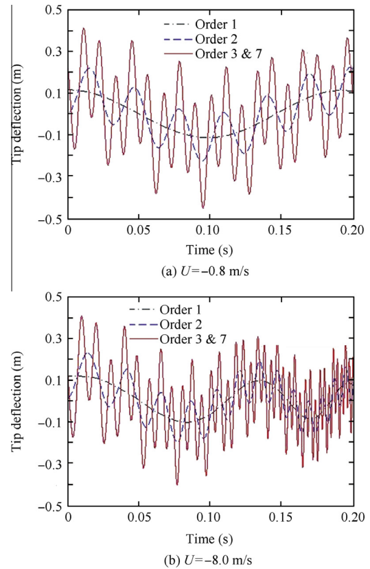
Fig. 4 Tip deflection response for the first 3 order initial conditions for L_0 = 3 \text{ m} .
