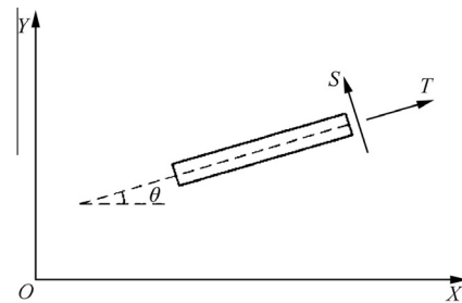
Fig. 3 Geometric diagram of coordinate transformation.
