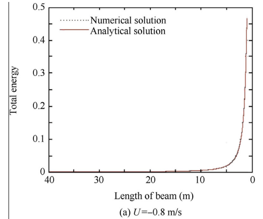
Fig. 9 Energy variation with length of beam.
