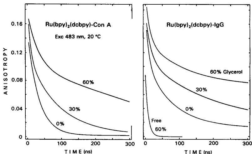
FIGURE 8 Viscosity-dependent anisotropy decays of [Ru(bpy)_2(dcbpy)] conjugated to ConA (left) and IgG (right).
