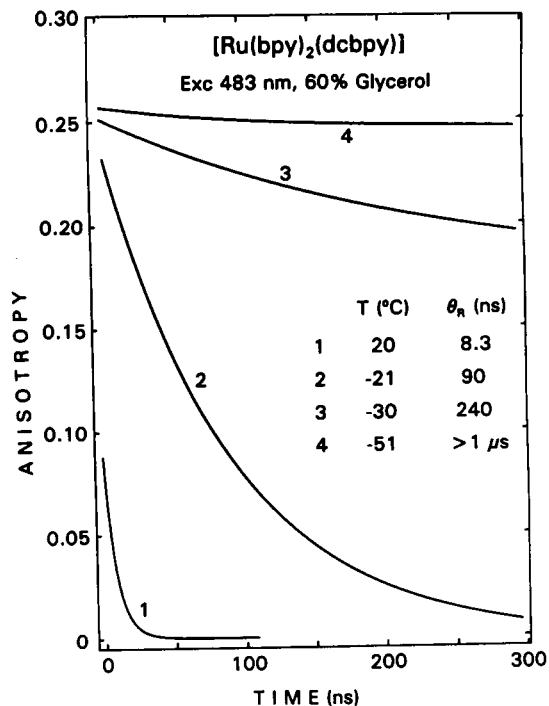
FIGURE 6 Anisotropy decays of free [Ru(bpy)_2(dcbpy)] in glycerol/water (60/40, v/v) at the indicated temperatures.
