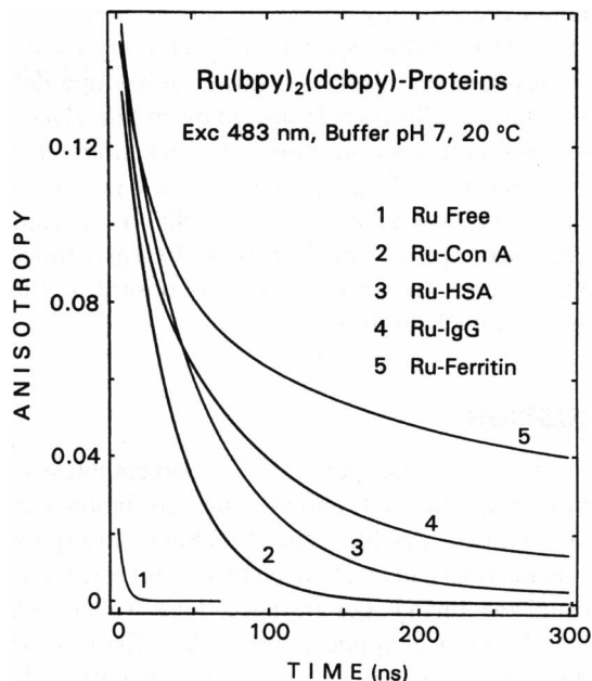
FIGURE 7 Anisotropy decays of [Ru(bpy)_2(dcbpy)] in buffer and conjugated to proteins.
