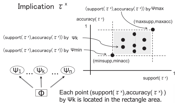
Fig. 1. Each pairs (support(\tau^x), accuracy(\tau^x)) in \psi (\psi \in DD(\Phi)) belongs to the rectangle area. In DIS , the minimum and the maximum points are the same, however they are different in NIS .
