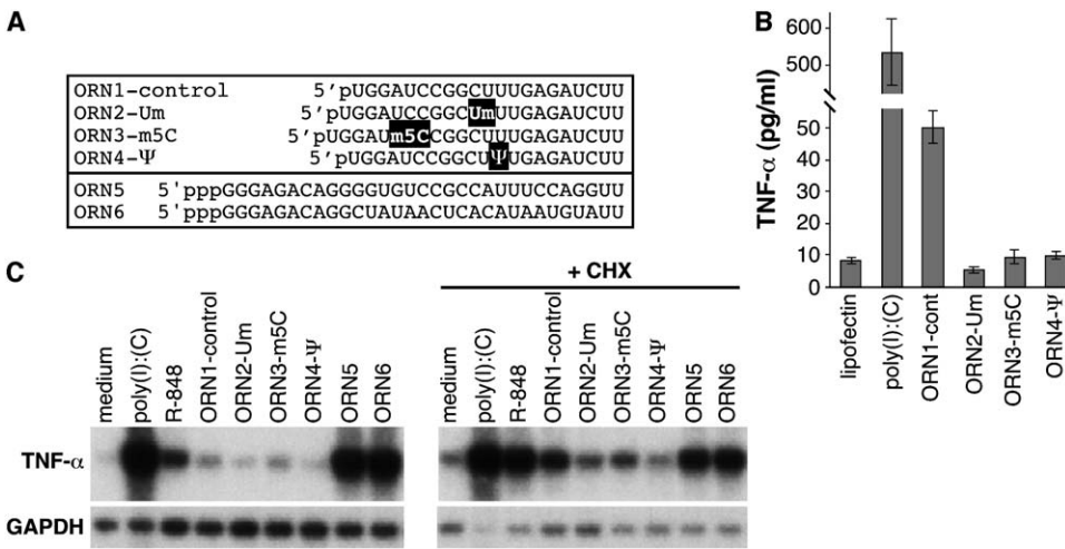
Figure 6. TNF- \alpha Expression by RNA-Transfected DCs (A) Sequences of oligoribonucleotides (ORNs) synthesized chemically (ORN1-4) or transcribed in vitro (ORN5-6) are shown. Positions of modified nucleosides Um (2'-O-methyluridine), m5C, and \Psi are highlighted. Human MDDCs were transfected with lipofectin alone (medium), R-848 (1 \mu g/ml), or with the indicated RNA (5 \mu g/ml) complexed with lipofectin. Where noted, cells were treated with 2.5 \mu g/ml cycloheximide (CHX). After 8 hr incubation, TNF- \alpha was measured in the supernatant by ELISA (B). Mean values \pm SEM are shown. The results are representative of three independent experiments. RNA isolated from the cells were analyzed by Northern blot (C).
