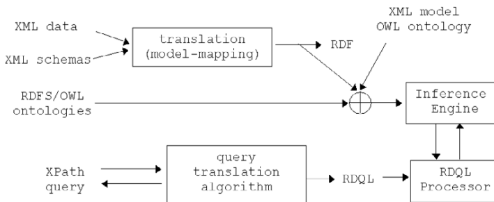
Fig. 1. Semantic XPath processor architecture overview
