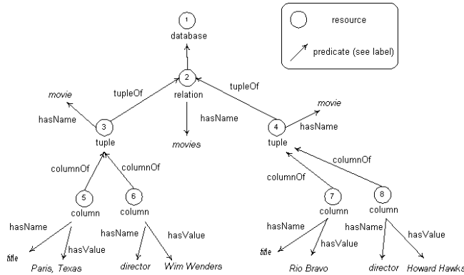
Fig. 4. RDF representation of the relational version of the movies example
