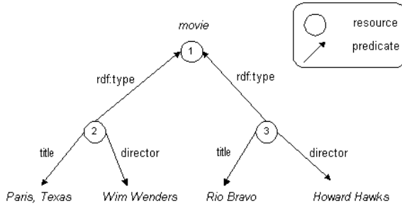
Fig. 5. Natural-RDF representation of the movies example
