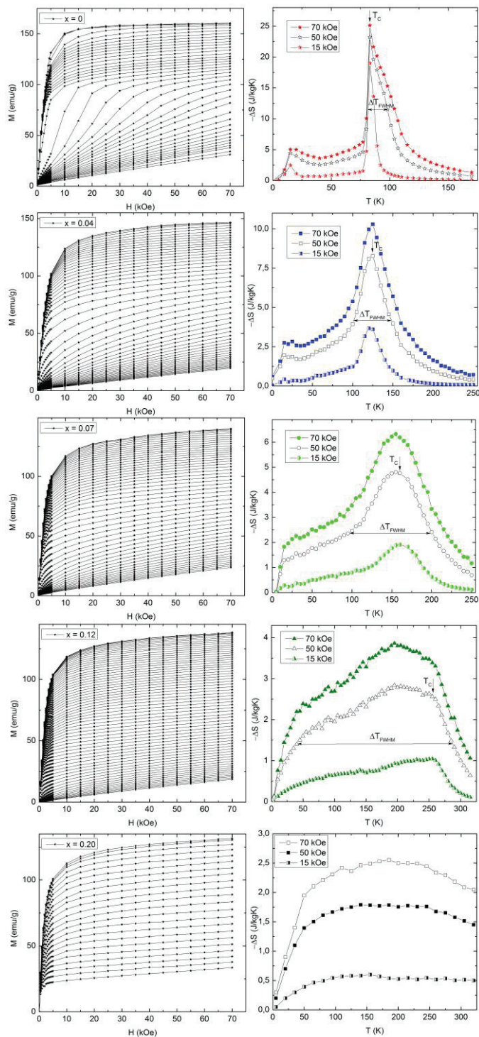
Figure. 7: Magnetization isotherms at various temperatures and magnetic entropy change temperature dependences -\Delta S(T) for \text{Ho}(\text{Co}_{1-x}\text{Fe}_x)_2 in different magnetic fields
