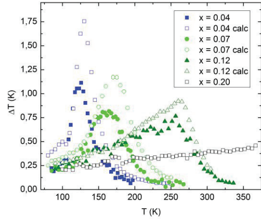
Figure. 8: Experimental and calculated using (4) MCE temperature dependencies ( \Delta T - effect) in \text{Ho}(\text{Co}_{1-x}\text{Fe}_x)_2 compounds
