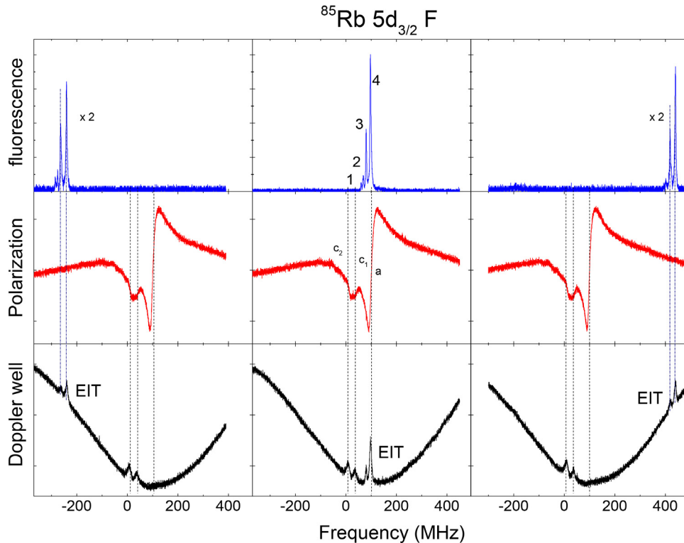
Figure 6. Fluorescence (top) and absorption (bottom) signals obtained with the 780 nm laser scanning across the Doppler broadened D2 line of ^{85}\text{Rb} and the frequency of the 776 nm laser passively stabilized to the Doppler shifted resonances of the 5\text{P}_{3/2} \rightarrow 5\text{D}_{3/2} manifold. The dispersion in the middle panel corresponds to the one-color polarization spectroscopy shown in block (A) of Figure 2. Saturated absorption features in the Doppler well can be identified with the D2 cycling transition (a) and cross-over ( c_1 and c_2 ) features in the one-color polarization spectra. A reduction in the absorption of the 780 nm light is observed whenever the Doppler shifts induced in both light components make a velocity group resonant with the two-photon transitions, producing also a fluorescence signal. Note that the relative height of the four fluorescence peaks depends on the position of these features across the Doppler well.
