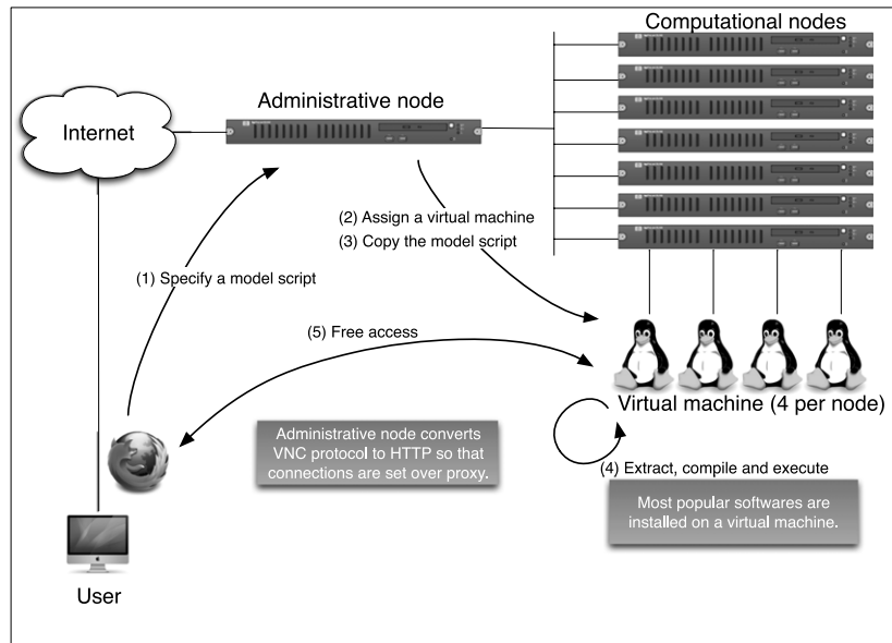
Fig. 2. Overall structure of Simulation Platform.
