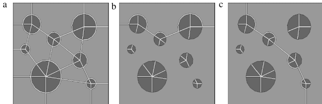
Fig. 21. Nooru-Mohamed test. Mesoscale cells with different cohesive-band patterns. (a) Original failure cell; (b) Failure cell allowing only a quasi-horizontal failure mechanism; (c) Failure cell allowing an oblique failure mechanism.
