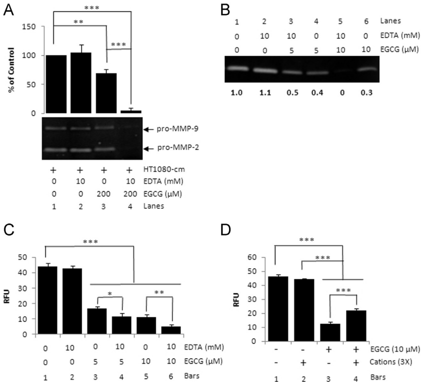
Fig. 2. Effect of divalent cations on inhibition of MMP-2 by EGCG. HT1080-cm (A) or purified active MMP-2 (B,C) was pretreated with EDTA before addition of EGCG at indicated concentrations. The mixtures were then analyzed by gelatin zymography (A,B) or FRET-peptide based fluorogenic substrate assay (C). (A) The bar graph is a quantitative representation of pro-MMP-2 activity (in %) relative to control. Bars represent mean \pm SD ( n=3 ). A representative zymogram is shown below. (B) A representative gelatin zymogram showing the effect of EDTA pretreatment on the activity of purified MMP-2. The numbers below the panel indicate relative MMP-2 activity in samples relative to control (set to 1). (C) Result of the FRET-peptide based fluorogenic substrate assay to study the effect of EDTA pretreatment on purified MMP-2 activity. Bars represent mean \pm SD ( n=3 ). (D) EGCG was first pretreated with 3-fold excess of divalent cations. The mixture was then added to purified active MMP-2 followed by analysis of MMP-2 activity by FRET peptide based assay. RFU – relative fluorescence units. * p < 0.05 , ** p < 0.01 , *** p < 0.001 .
