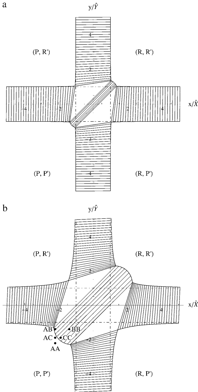
FIGURE 1 (a) Phase diagram in the x,y plane of the bilayer for r = 1 , so that the leaves are essentially identical, and a weak coupling \beta = 0.5 . The order parameter, y , of the outer leaf is shown in units of \hat{Y} , and that of the inner leaf, x , is shown in units of \hat{X} = r\hat{Y} . The tie lines end on the binodals of the coupled system shown with solid lines. The dashed-dotted lines denote the binodals of the uncoupled system. There are four possible phases of the bilayer; one in which the order parameters in both leaves are positive, (R,R') , one in which they are both negative, (P,P') , and two phases in which the order parameter in one leaf is positive while that in the other leaf is negative. Note that the region of four-phase coexistence in the uncoupled system breaks into two regions of three-phase coexistence connected by a region of two-phase coexistence between (R,R') and (P,P') . (b) Phase diagram in the x,y plane of the bilayer for r = 1 , and a stronger coupling \beta = 3.0 . The point AA represents the state of a bilayer which consists of coupled, identical, leaves such that the system is in the one-phase region (P,P') ; BB represents a bilayer of coupled, identical, leaves of a different composition such that the system is well within the coexistence region between (R,R') and (P,P') ,
